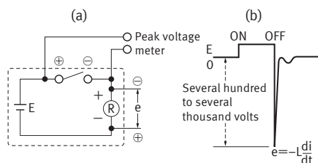
Fig. 13 Example of counter emf and actual measurement
