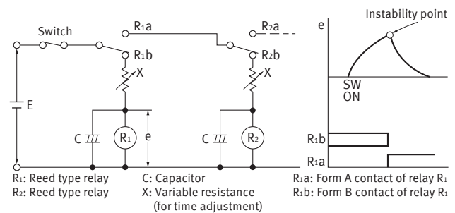
Fig. 7 " Not a good example " : A timing and sequential operation using a reed type relay
