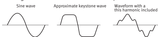
Fig. 1 Distortion in an AC stabilized power source
