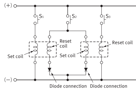
( c ) Parallel connection of set coils and reset coils
