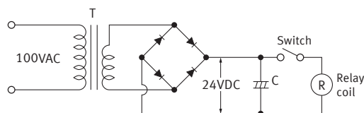
Fig. 2 Voltage fluctuation absorbing circuit using a condenser
