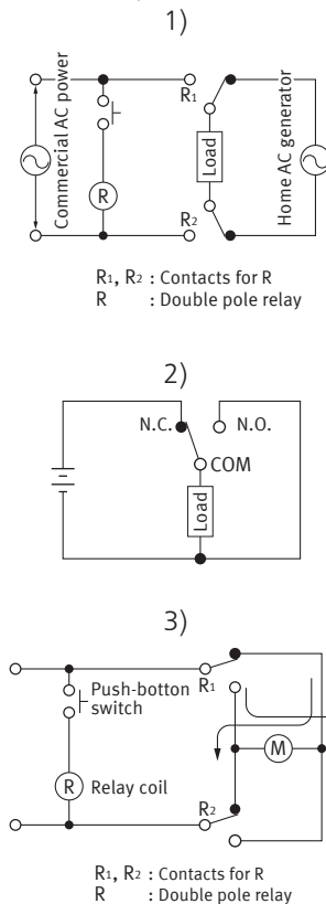
Fig. 16 Bad example of Form A and B use
