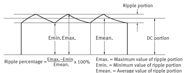
Fig. 4 Applied voltage and voltage drop of the coil
