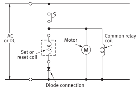
( d ) Circuit with inductive load in parallel with the set coil or reset coil
