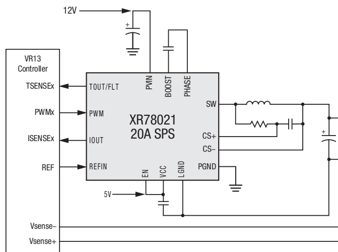
XR78021 Typical Application
