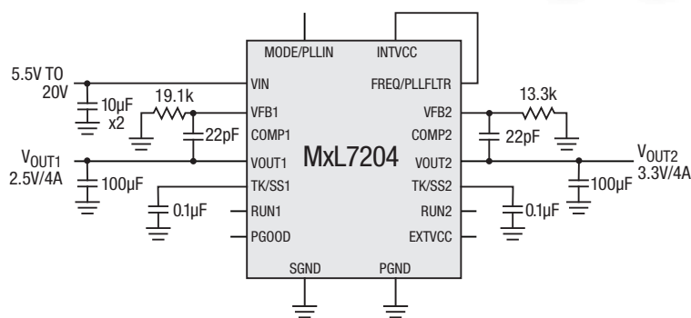
Typical Application
