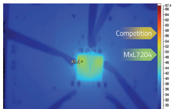
MxL7204 Thermal Image
