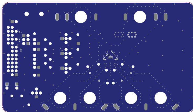
MAX98415A/MAX98425A DEV Board PCB Layout—Inner Layer 1
