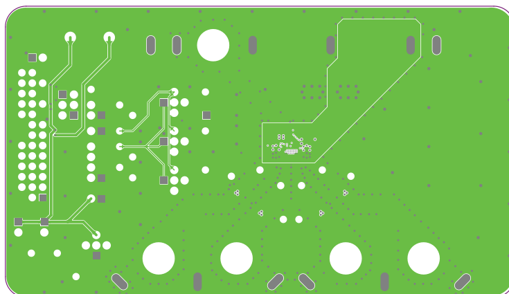
MAX98415A/MAX98425A DEV Board PCB Layout—Inner Layer 3
