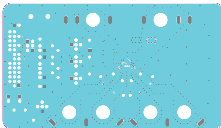
MAX98415A/MAX98425A DEV Board PCB Layout—Inner Layer 4
