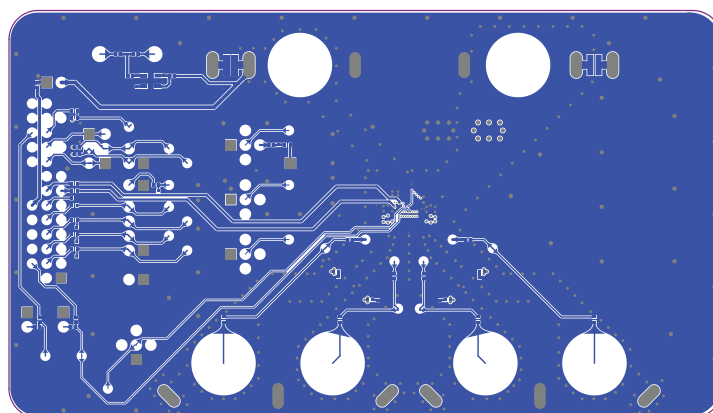
MAX98415A/MAX98425A DEV Board PCB Layout—Bottom Layer
