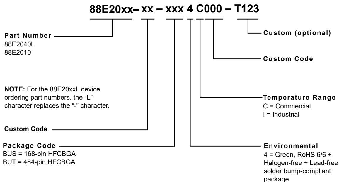
Figure 42: Sample Part Number
