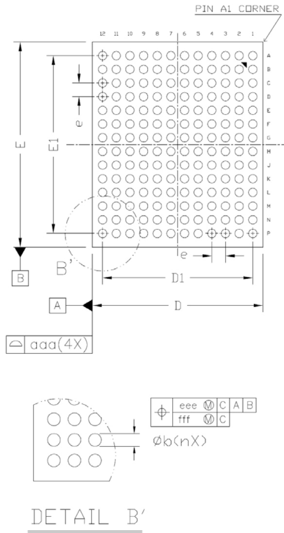
Figure 39: 168-pin 10 mm x 12 mm HFCBGA Bottom View
