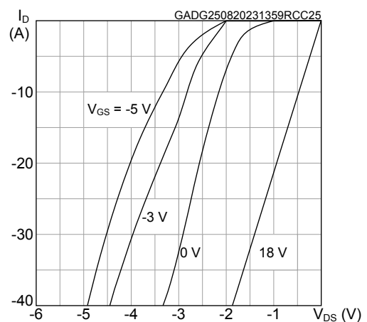
Figure 8. Typical reverse conduction characteristics ( T_J = 25^\circ\text{C} )
