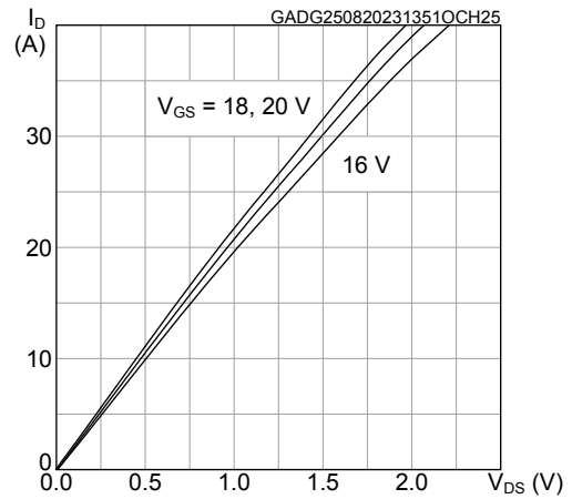
Figure 4. Typical output characteristics ( T_J = 25^\circ\text{C} )
