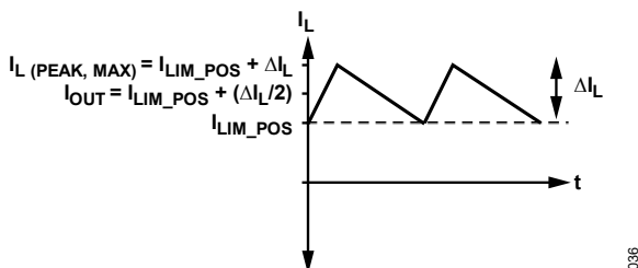
Figure 34. Positive Valley Current Limit
