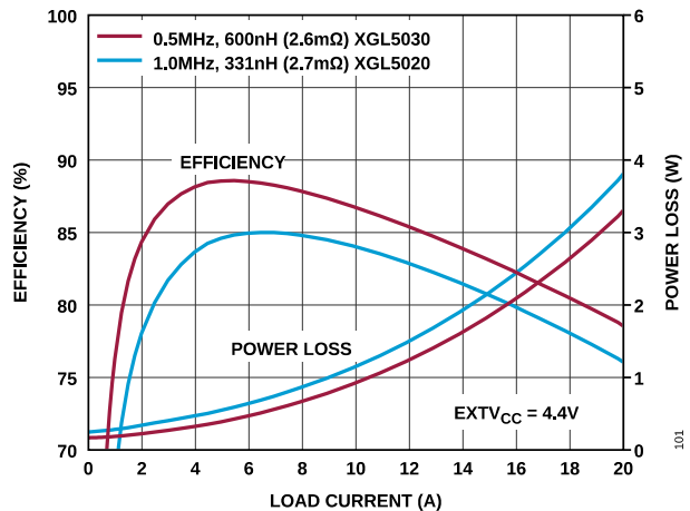
Figure 9. LT7171-1 12V IN to 0.6V OUT Efficiency
