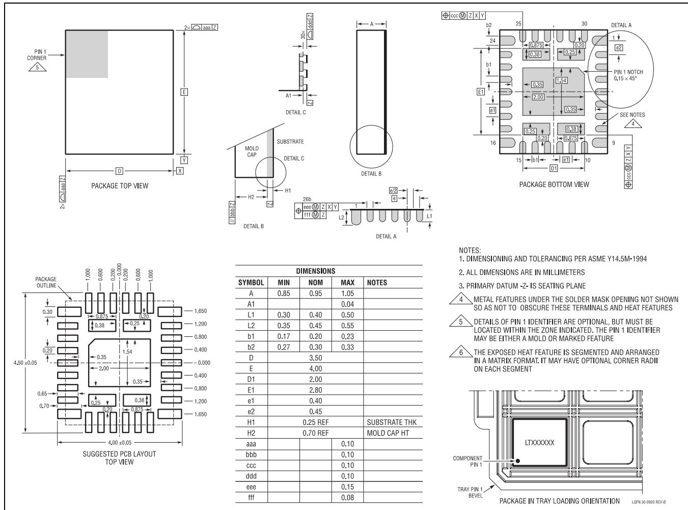
Figure 44. 30-lead (3.5mm x 4mm) LQFN Package (05-08-7066) Dimensions shown in millimeters
