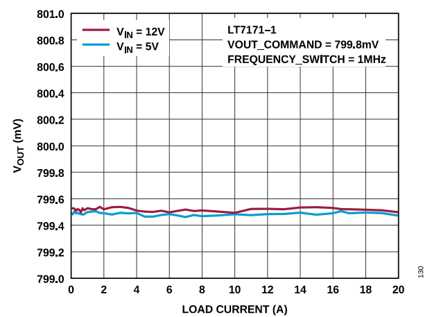
Figure 15. Load Regulation
