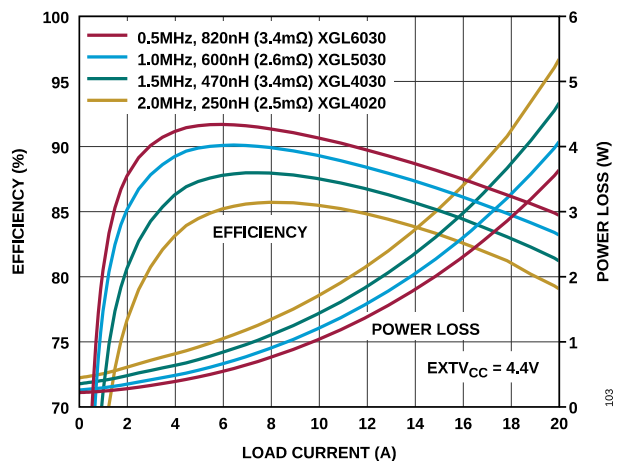
Figure 11. LT7171-1 12V IN to 1.0V OUT Efficiency
