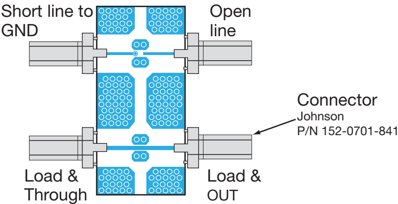
Calibration Jig
