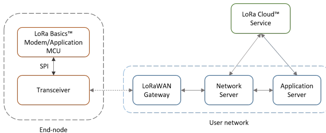
Fig. 3.1: LoRa Basics™ Modem Network Architecture
