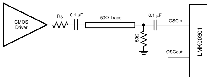
Figure 18. Driving OSCin With a Single-Ended Input
