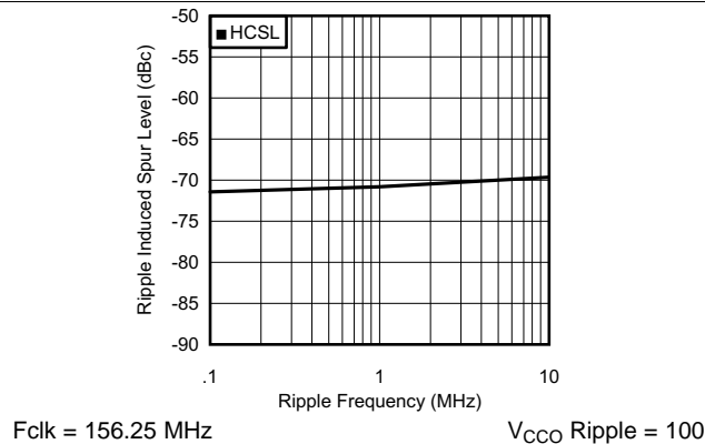
Figure 7. PSRR vs Ripple Frequency at 156.25 MHz
