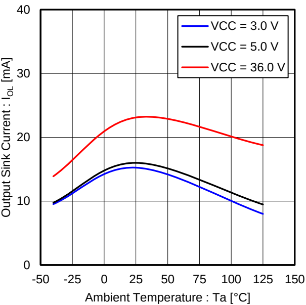
Figure 6. Output Sink Current vs Ambient Temperature ( V_{OUT} = 1.5\text{ V} )
