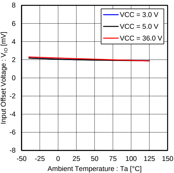
Figure 8. Input Offset Voltage vs Ambient Temperature
