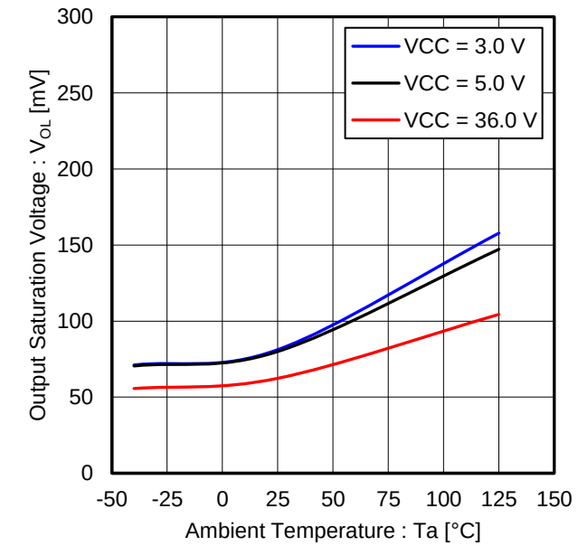
Figure 4. Output Saturation Voltage vs Ambient Temperature (I OL = 4 mA)
