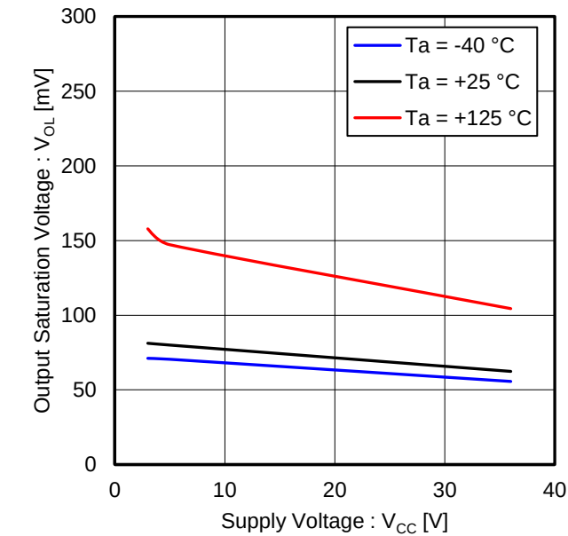
Figure 3. Output Saturation Voltage vs Supply Voltage (I OL = 4 mA)
