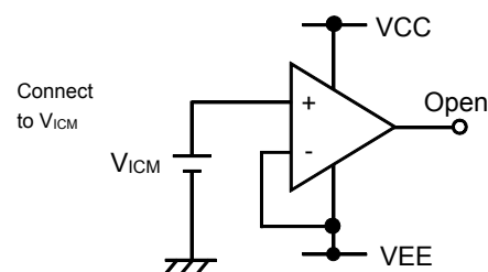
Figure 20. Example of application unused circuit processing
