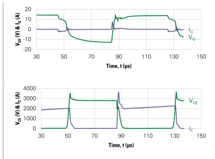
(b) Waveforms – T2000BB45G, T_j = 125^\circ\text{C} , V_{CE} = 2800 V, I_c = 2000 A, di/dt = 3500 A/ \mu\text{s}
