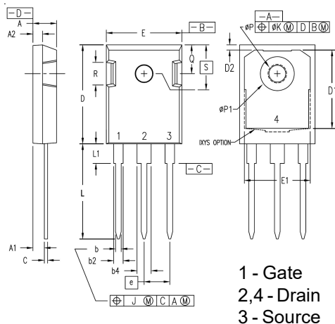
TO-247 Outline
