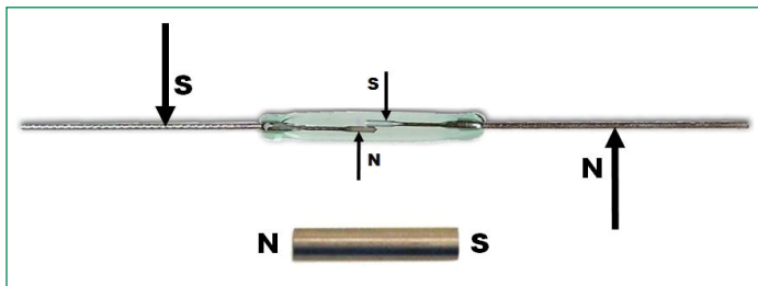
Figure 1. Magnetic Induction
