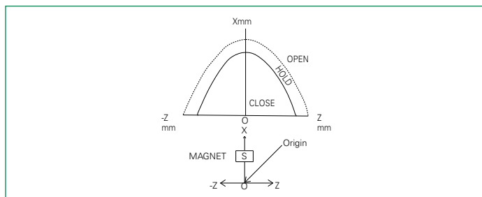
Figure 3. Magnet Parallel to Reed Switch
