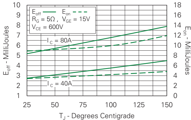
Fig. 15. Inductive Switching Energy Loss vs. Junction Temperature
