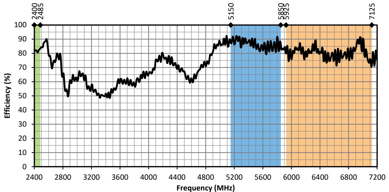
Figure 8. ANT-W63WS2-ccc Antenna Efficiency, Straight
