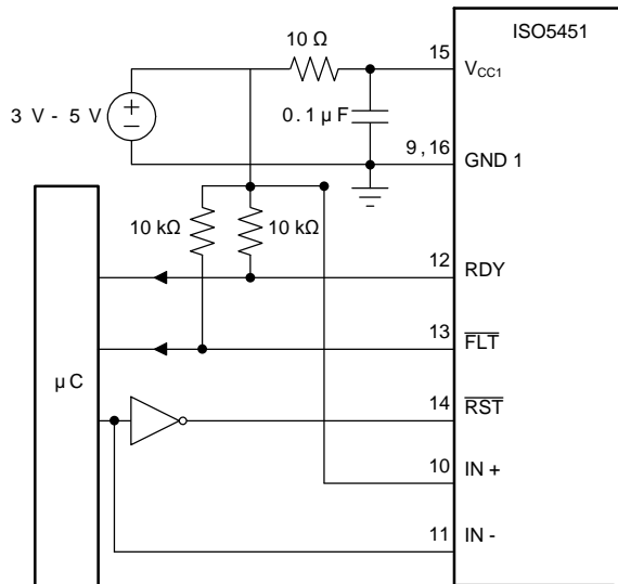
Figure 48. Auto Reset for Noninverting and Inverting Input Configuration
