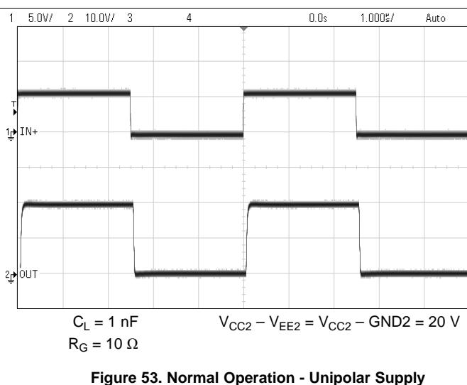
Figure 53. Normal Operation - Unipolar Supply
