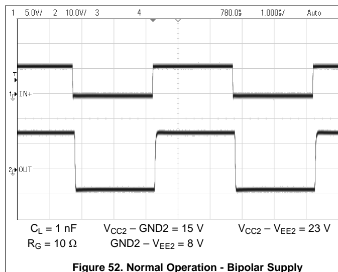
Figure 52. Normal Operation - Bipolar Supply
