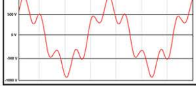
Figure 3: Harmonic rich waveform
