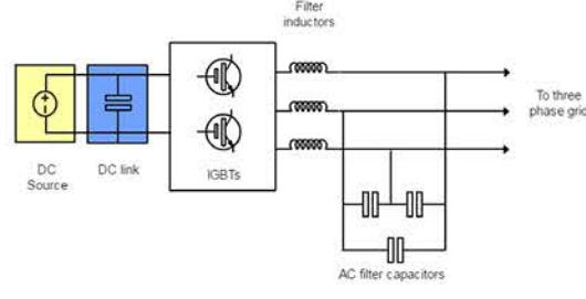
Figure 1: Typical Inverter Block Diagram with output filter capacitors
