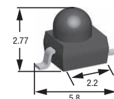
1.8 mm Gullwing
