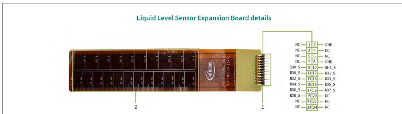
Figure 8 Liquid-level sensor expansion board
