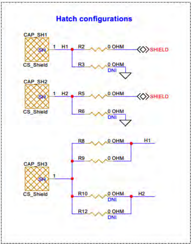
Figure 58 CAPSENSE™ hover-touch board shield configurations schematic
