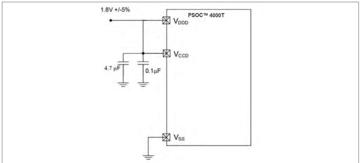
Figure 21 PSOC™ 4000T device schematic with 1.8 V ±5% external supply
