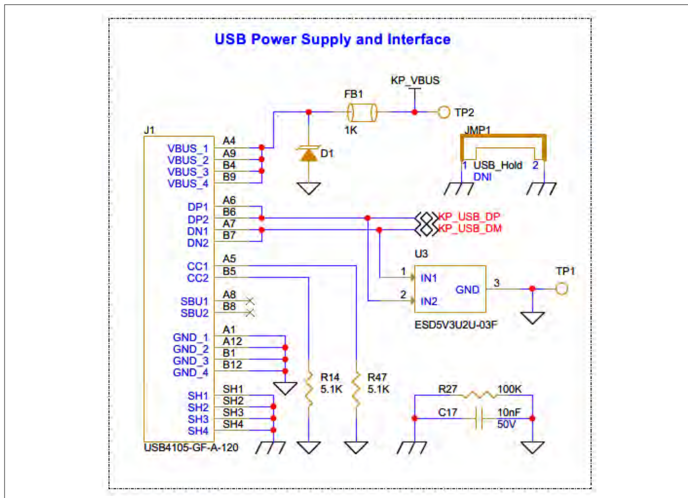
Figure 33 Schematic of the USB Type-C connector (J1) and ESD protection (D1, U3)
