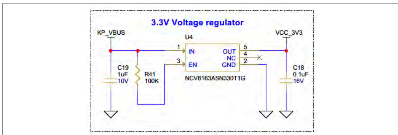
Figure 34 Schematic of the 3.3 V voltage regulator (U4)
