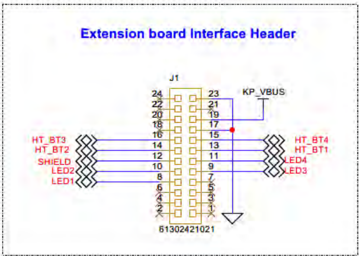
Figure 59 Expansion header interface schematic
