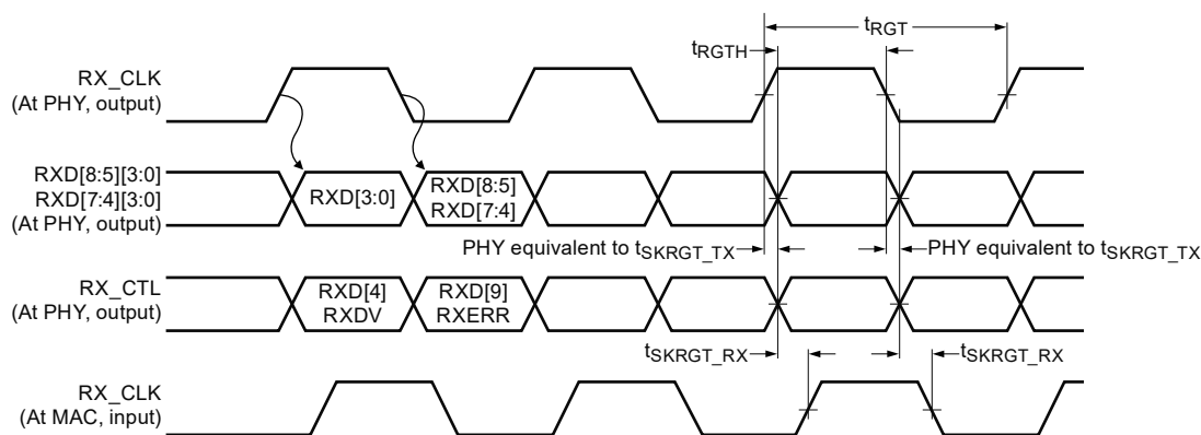
Figure 34. Receive timing and multiplexing diagram
