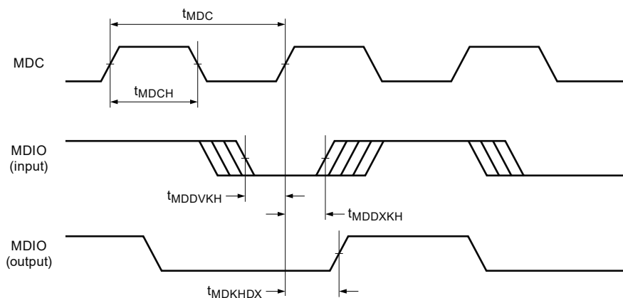
Figure 30. Ethernet management interface timing diagram
