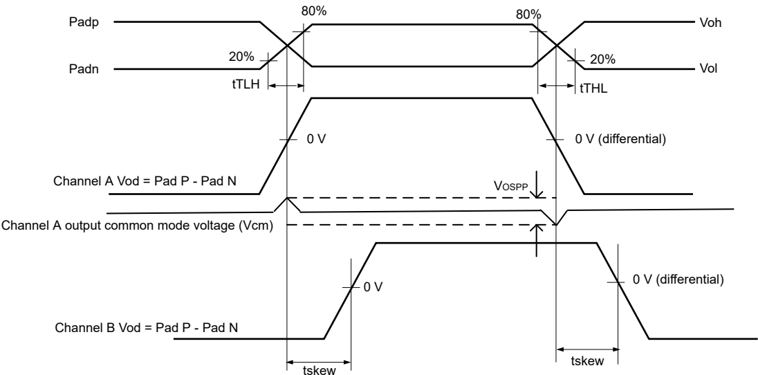
Figure 9. Output transition time waveform
