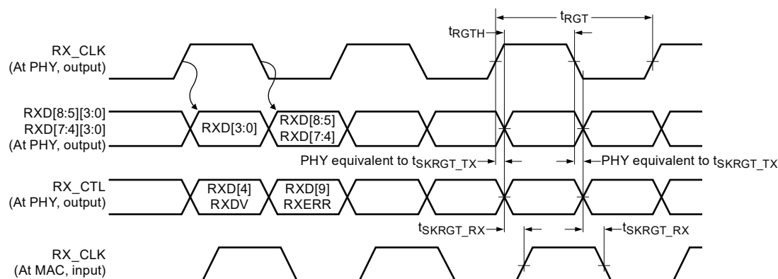
Figure 34. Receive timing and multiplexing diagram
