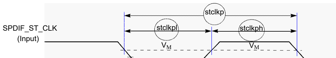
Figure 18. SPDIF_ST_CLK timing diagram
