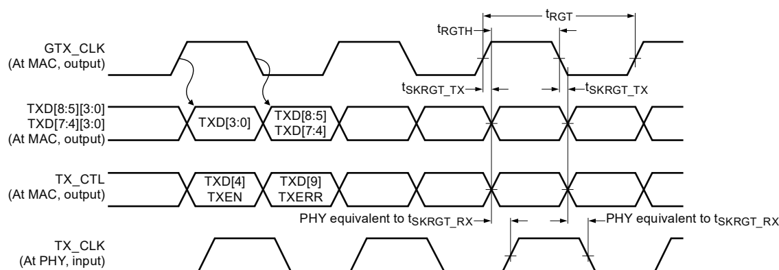
Figure 33. AC Transmit timing and multiplexing diagrams
