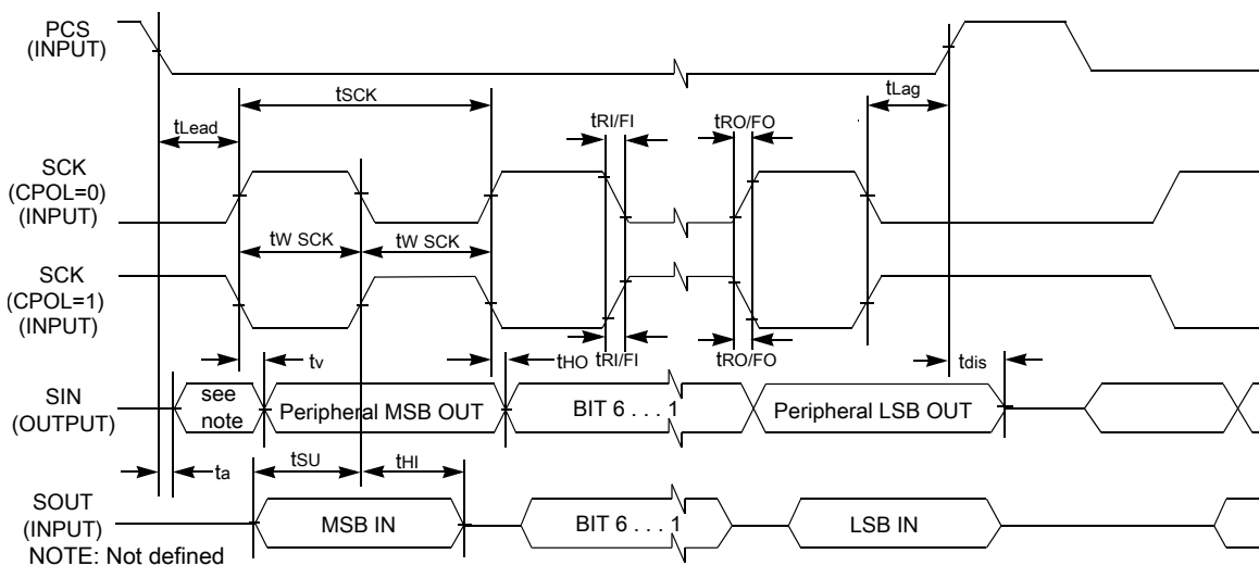
Figure 45. LPSPI Peripheral mode timing (CPHA = 1)
