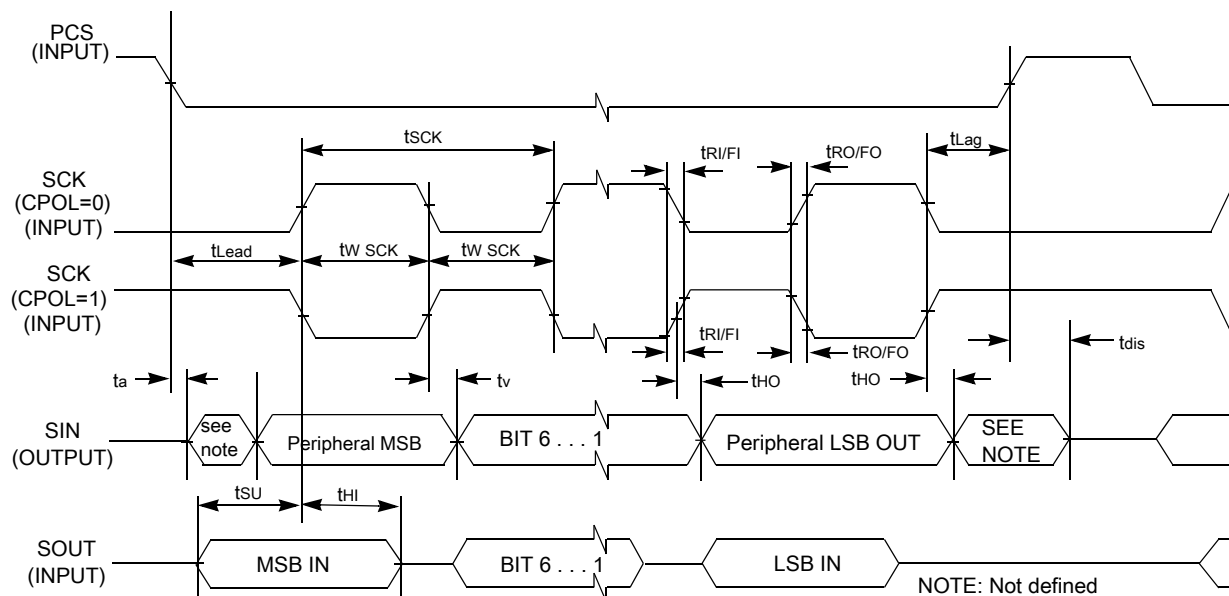
Figure 44. LPSPI Peripheral mode timing (CPHA = 0)
