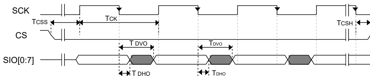
Figure 51. FlexSPI output timing in SDR mode
