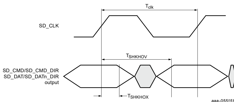
Figure 28. uSDHC AC HS400 timing
