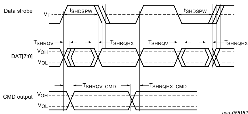
Figure 29. uSDHC AC HS400 timing 1
