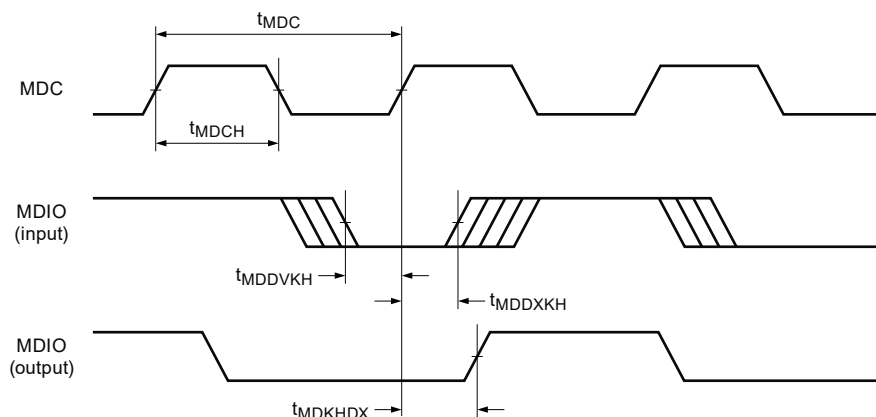
Figure 30. Ethernet management interface timing diagram
