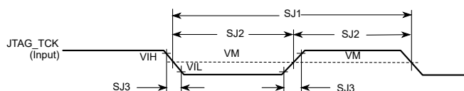
Figure 11. Test Clock Input Timing Diagram
