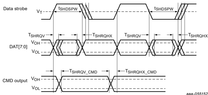
Figure 29. uSDHC AC HS400 timing 1
