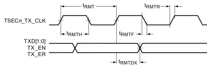
Figure 35. Transmit AC timing diagram
