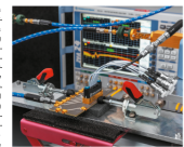
Fig.1 Example of a test setup for Design Validation Testing (DVT) with network analyzer and/or scope
