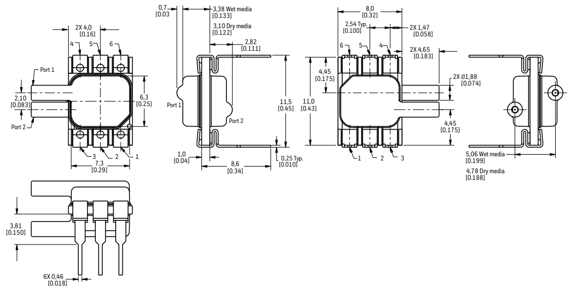
DIP JJ: Dual radial barbless ports, same side
