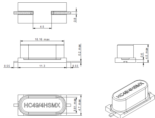
Outline (mm)
