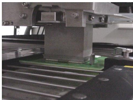
Reflow Nozzle
