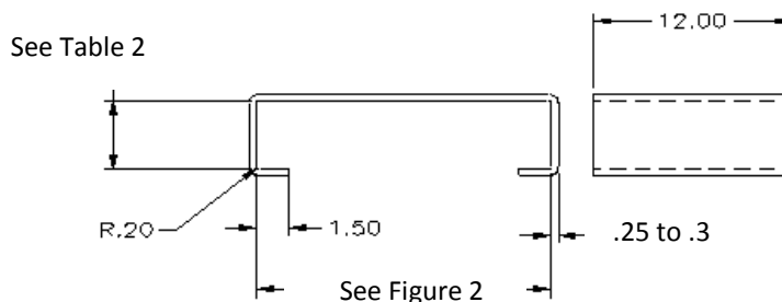
Figure 8: Rework Clip Dimensions are in MM
