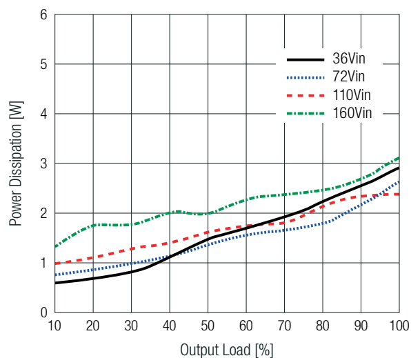
Power Dissipation vs. Output Current
