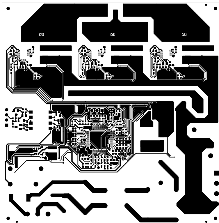
Figure 12. EVSTDRVG611MC layout - top layer
