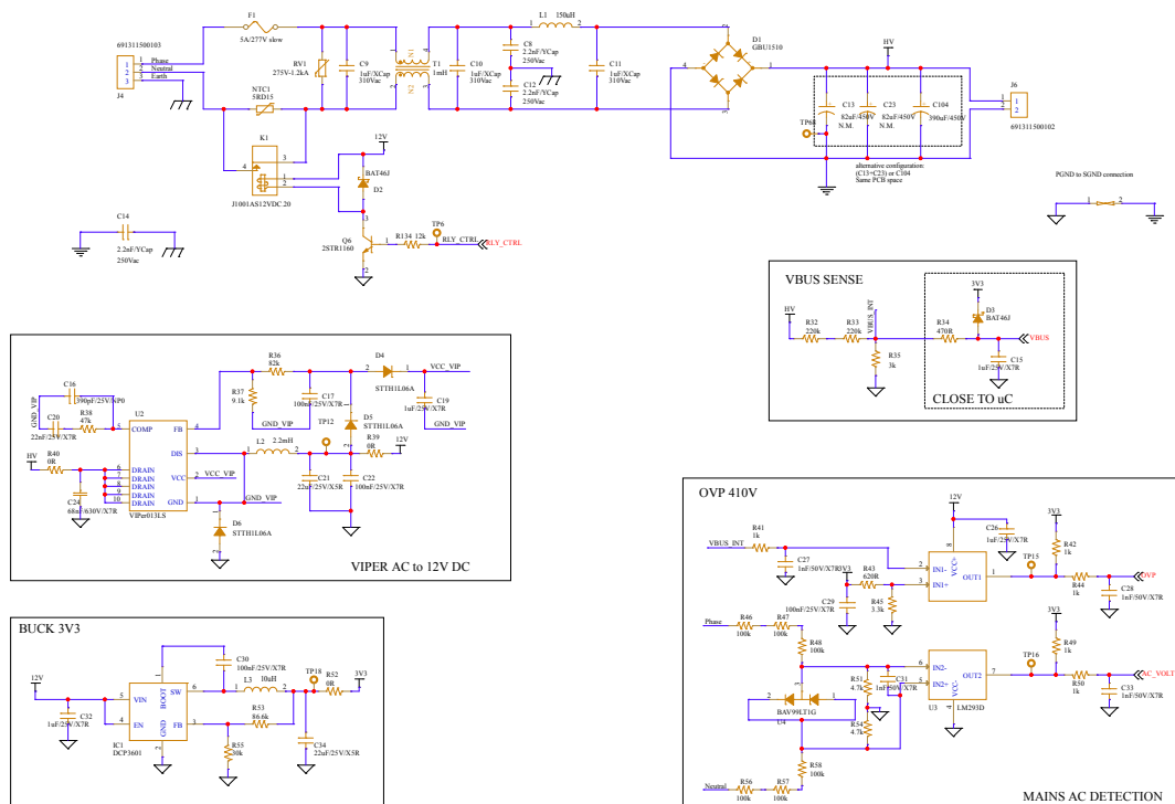
Figure 2. EVSTDRVG611MC schematic - power supply
