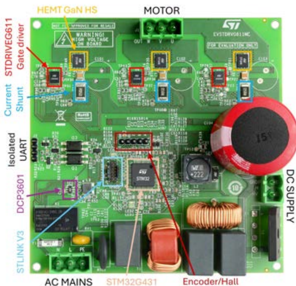
Figure 8. EVSTDRVG611MC top view connectors and components
