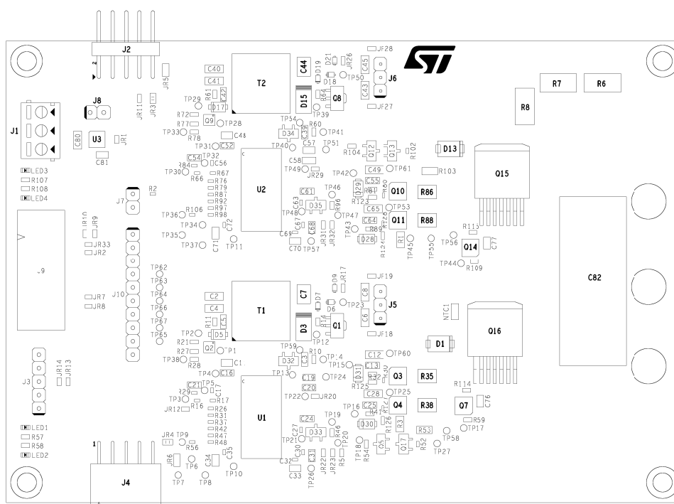
Figure 9. EVALSTGAP4S – Layout – TOP components placement
