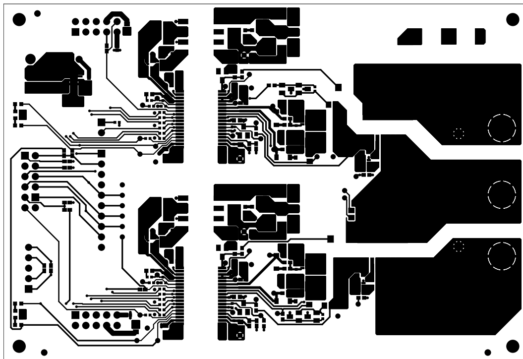
Figure 5. EVALSTGAP4S – Layout – Top layer
