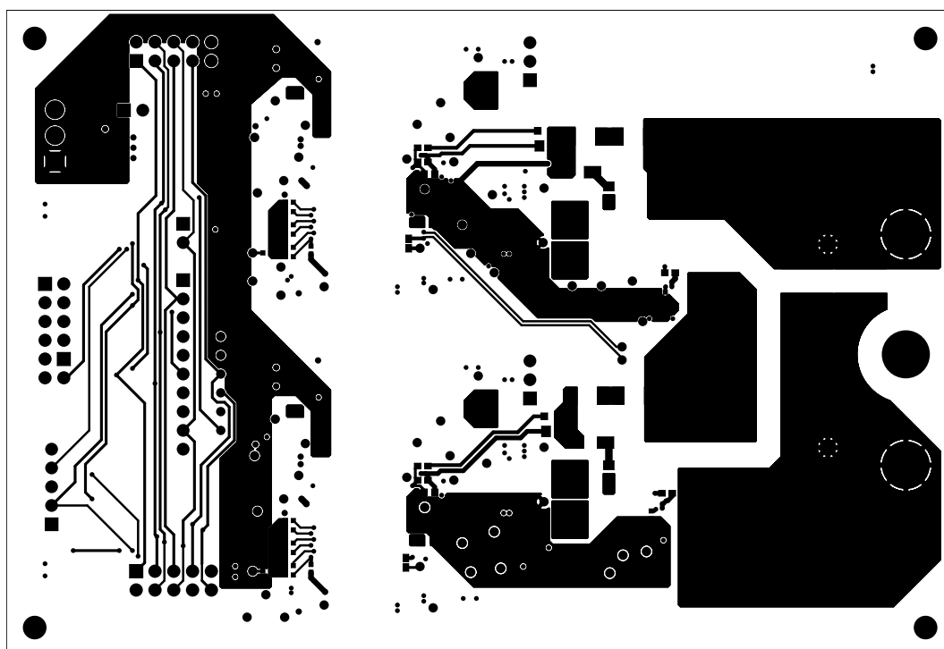
Figure 8. EVALSTGAP4S – Layout – Bot layer
