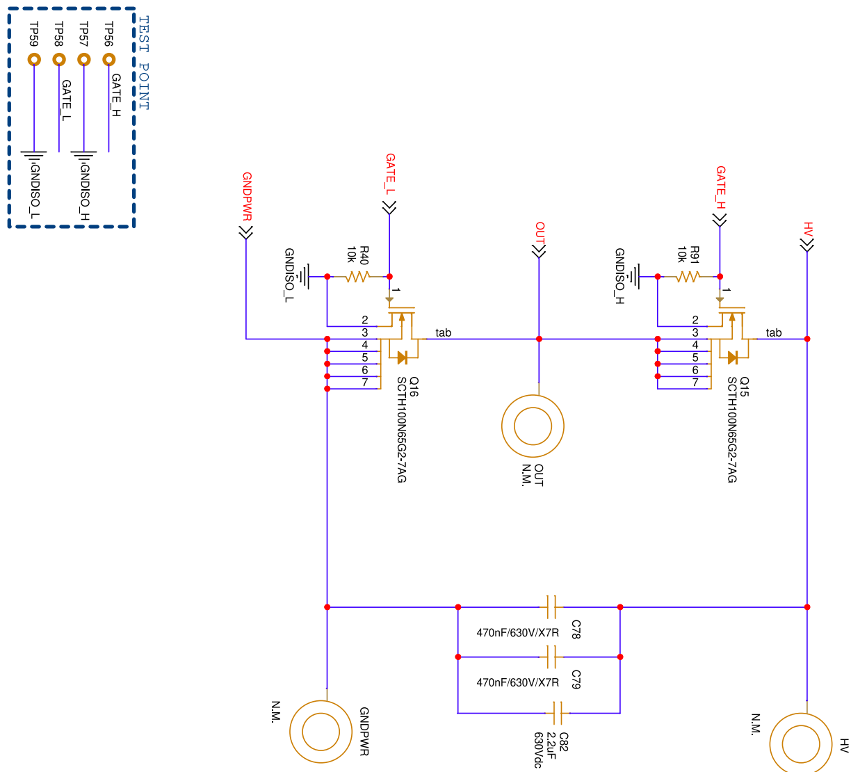
Figure 4. EVALSTGAP4S schematic diagram – power stage
