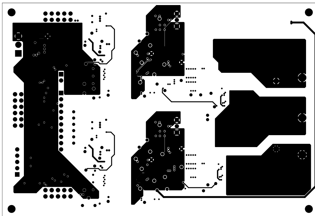
Figure 6. EVALSTGAP4S – Layout – Inner 1 layer
