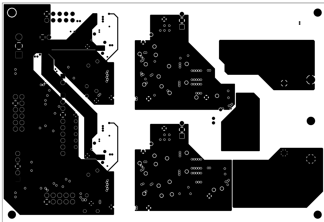
Figure 7. EVALSTGAP4S – Layout – Inner 2 layer
