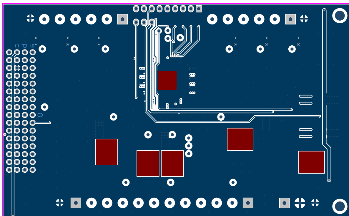
Figure 6. EVAL-L99UDL01 daughterboard bottom layer
