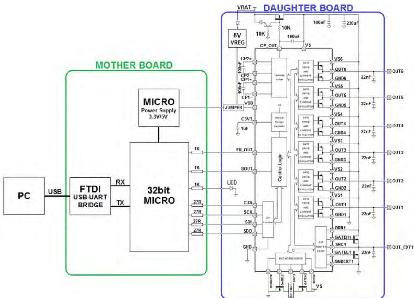
Figure 1. L99UDL01 evaluation board overall application diagram
