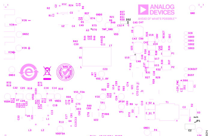
Figure 21. EVAL-ADAQ4224-FMCZ Silkscreen, Top Layer
