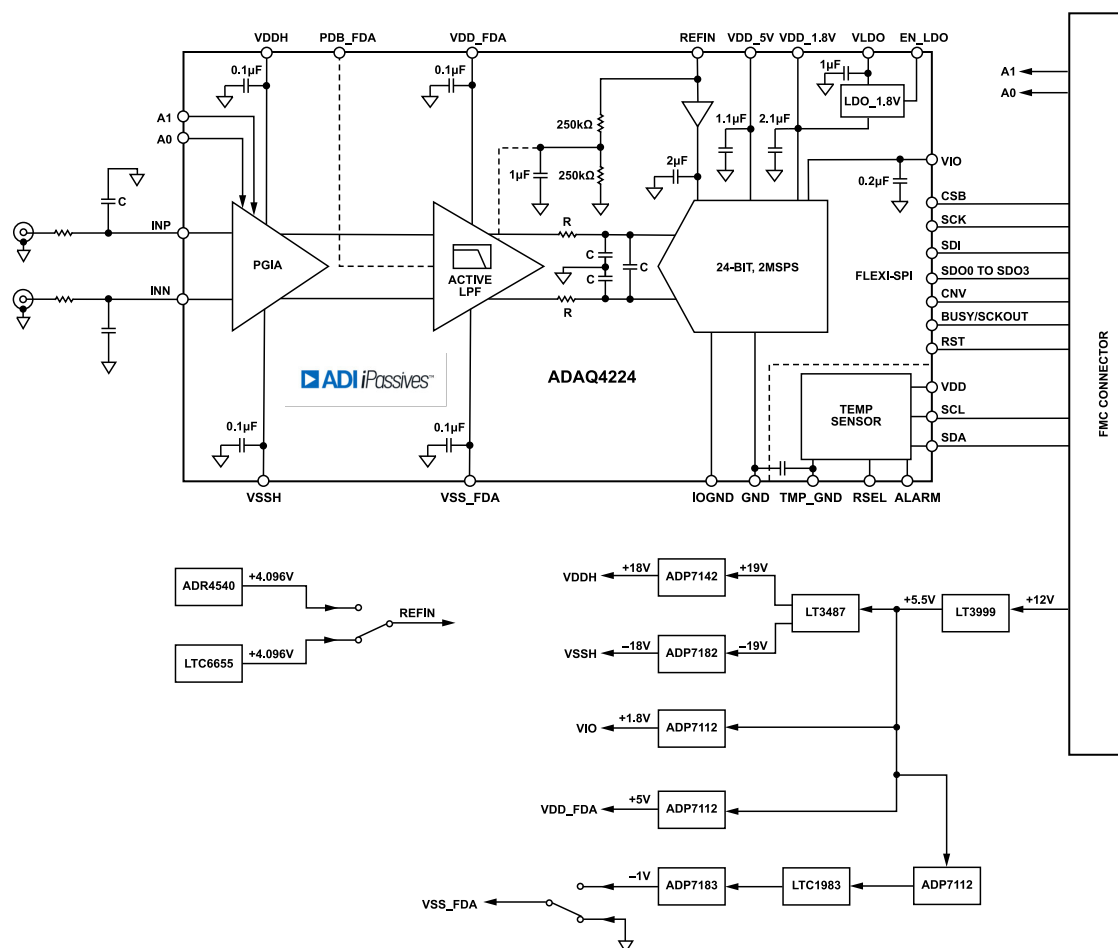
Figure 2. Simplified Evaluation Board Block Diagram
