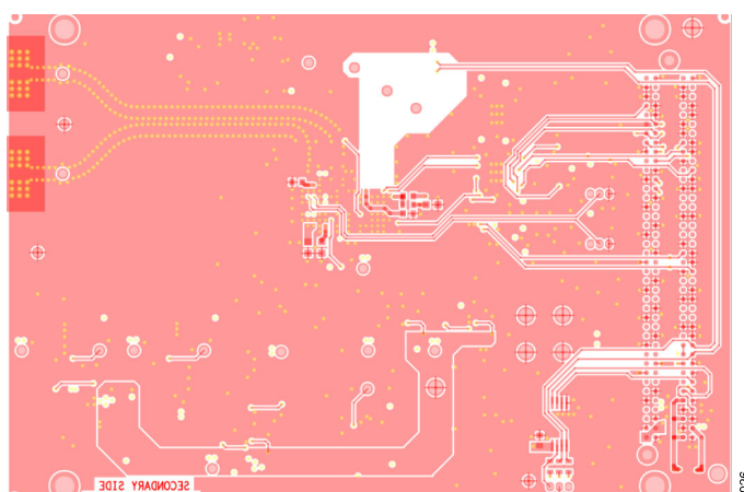
Figure 26. EVAL-ADAQ4224-FMCZ, Bottom Layer 4
