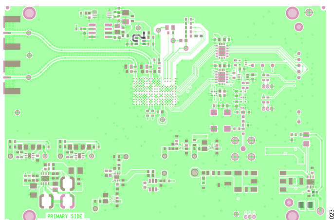
Figure 23. EVAL-ADAQ4224-FMCZ, Top Layer 1
