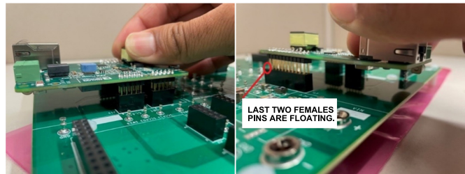
Figure 3. Alignment of an EVAL-10BT1L-MCS-AZ/EVAL-10BT1L-MCS-BZ shield with SPoE PSE Motherboard
