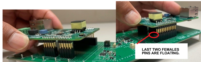
Figure 4. Alignment of an EVAL-10BT1L-MCS-AZ/EVAL-10BT1L-MCS-BZ shield with the SPoE PD Motherboard
