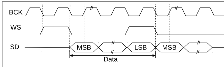
Figure 9-20. PCM Standard
