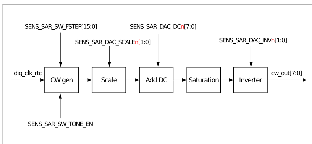
Figure 30-6. Workflow of CW Generator
