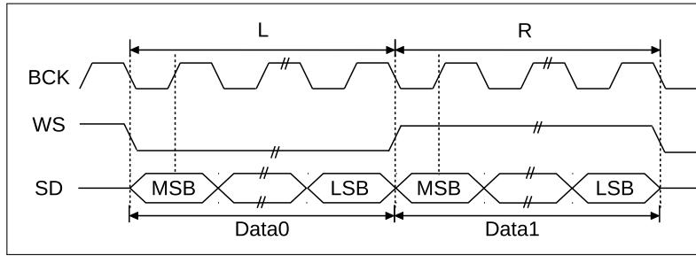
Figure 9-19. MSB Alignment Standard
