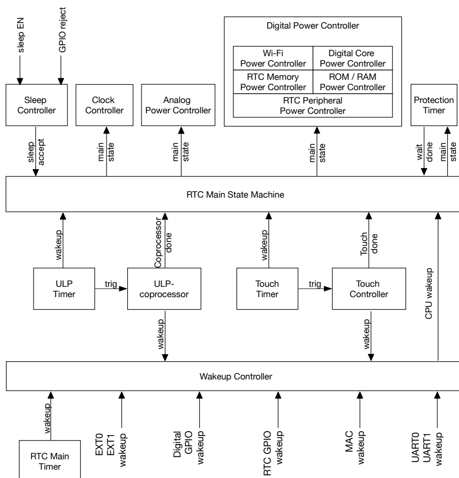
Figure 32-2. Power Management Unit Workflow
