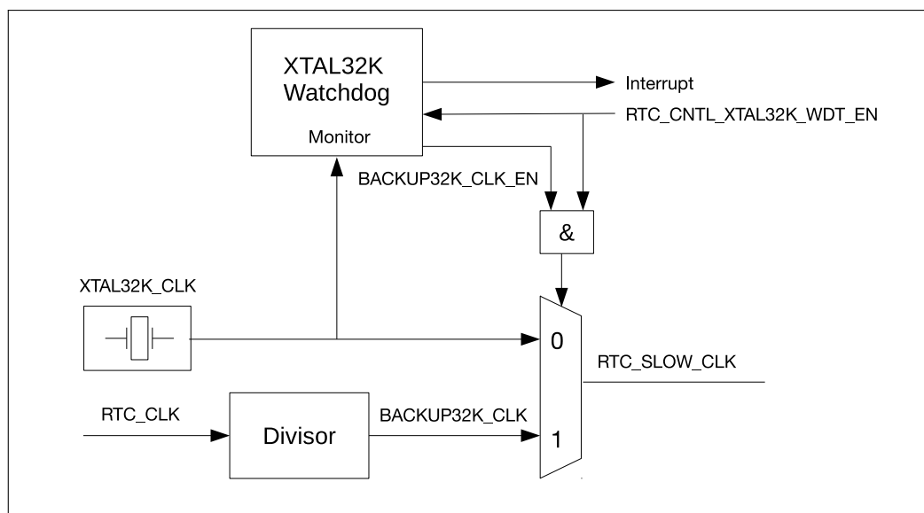
Figure 16-1. XTAL32K Watchdog
