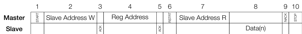
Figure 31-25. I2C Read Operation
