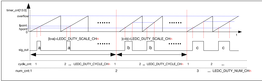
Figure 11-5. Output Signal Diagram of Fading Duty Cycle
