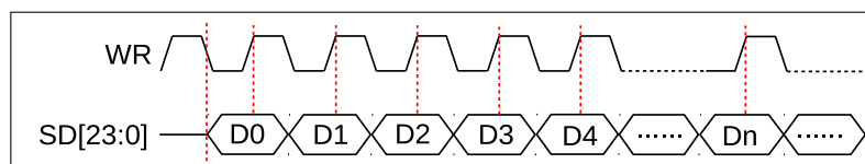
Figure 9-29. Data Frame Format 1 in LCD Master Transmitting Mode
