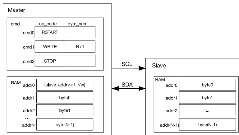
Figure 19-5. An I2C Master Writing to an I2C Slave with a 7-bit Address
