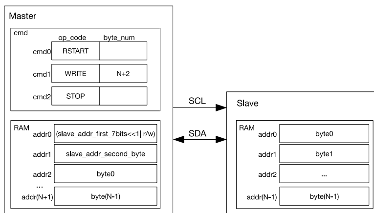
Figure 19-6. A Master Writing to a Slave with a 10-bit Address
