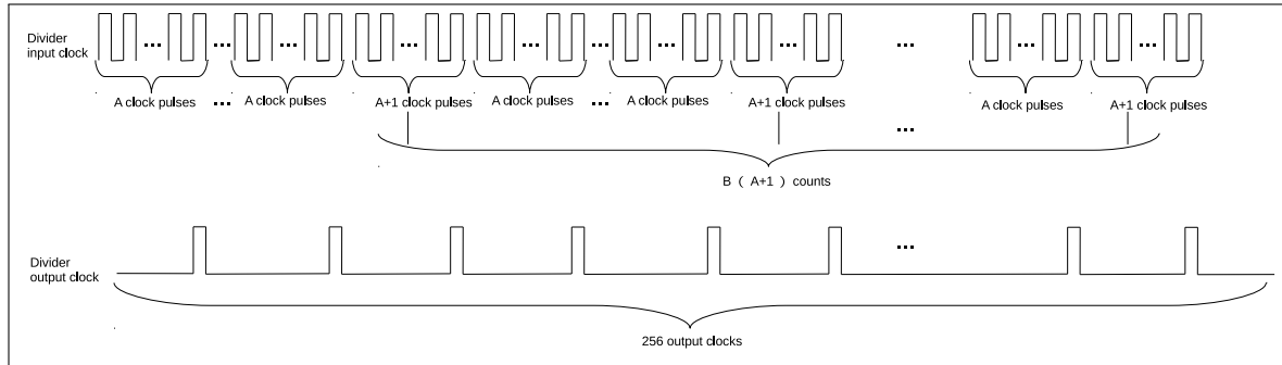
Figure 11-3. LED_PWM Divider
