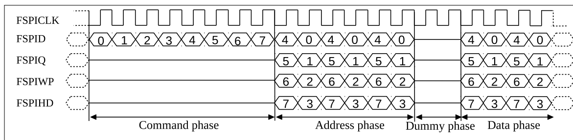
Figure 8-6. SPI Quad Read Command Sequence Sent by GP-SPI2 to Flash
