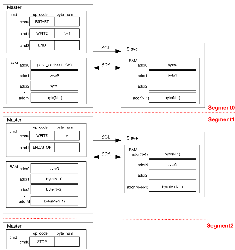
Figure 19-8. An I2C Master Writing to an I2C Slave with a 7-bit Address in Multiple Sequences
