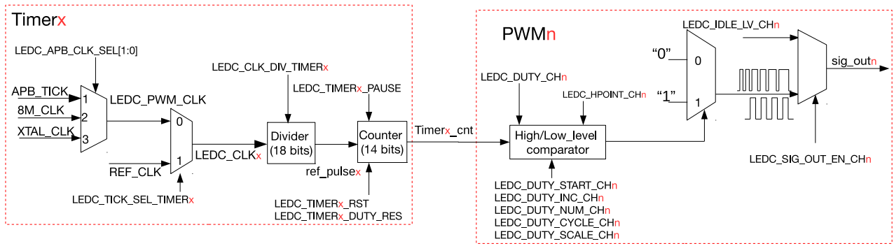
Figure 11-2. LED_PWM generator Diagram
