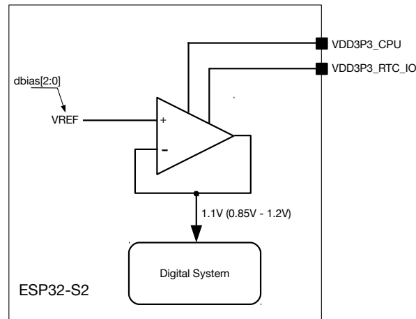
Figure 32-6. Digital System Regulator
