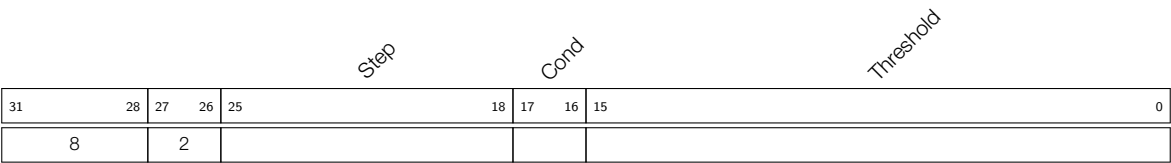
Figure 31-17. Instruction Type - JUMPS
