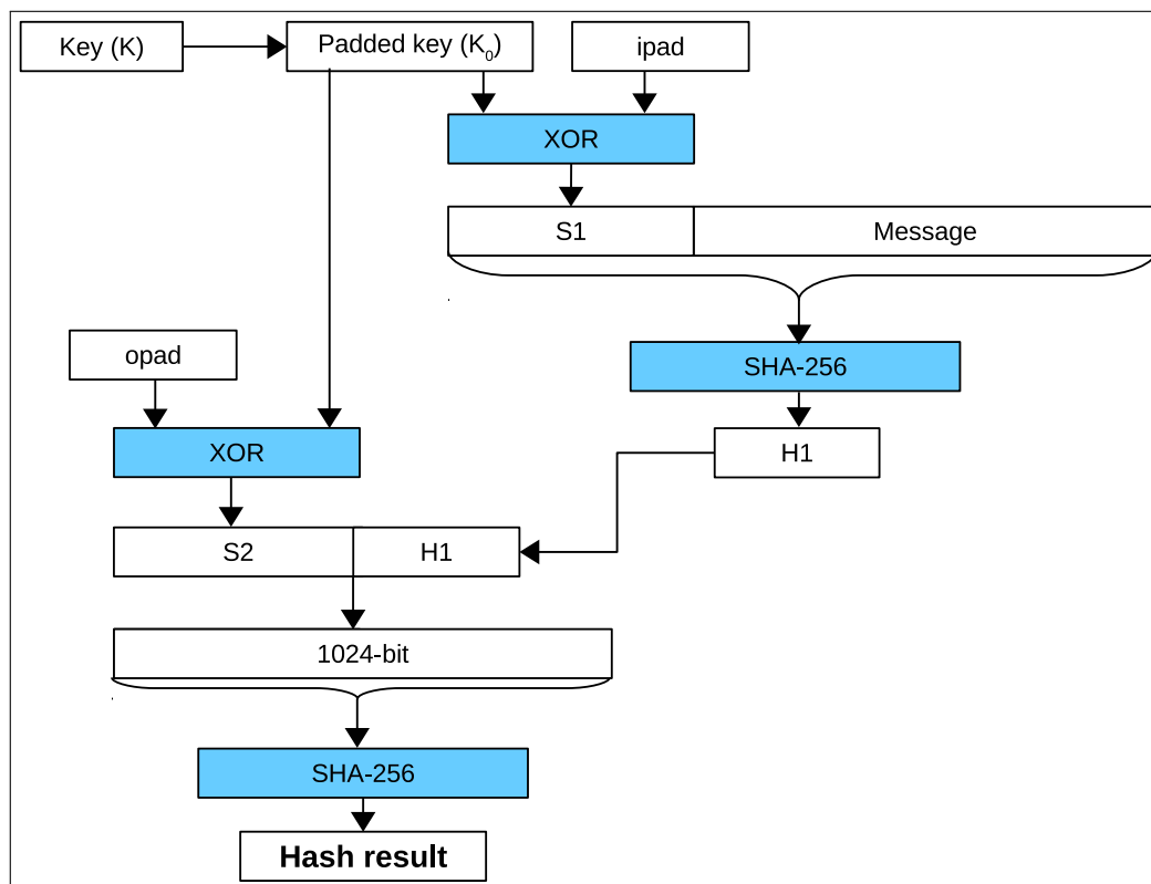
Figure 29-2. HMAC Structure Schematic Diagram
