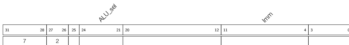
Figure 31-9. Instruction Type — ALU for Operations with Stage Count Register
