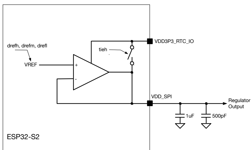
Figure 32-8. Flash voltage regulator
