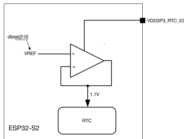
Figure 32-7. Low-power voltage regulator
