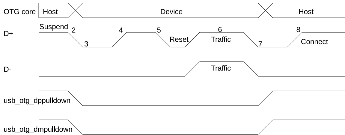
Figure 20-9. A-Device HNP
