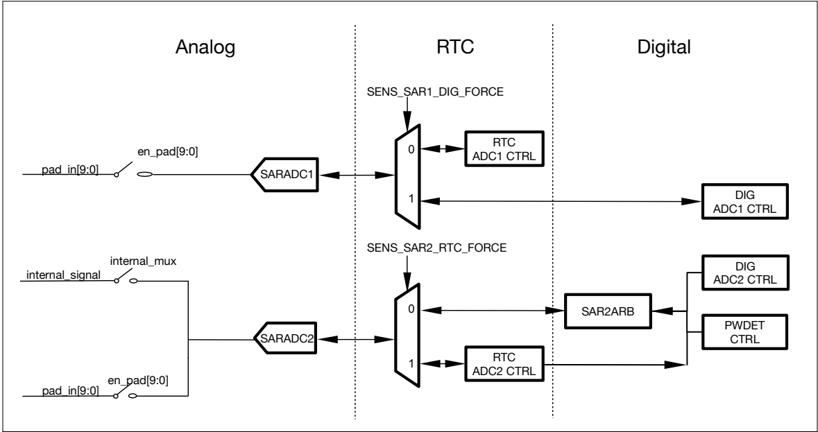
Figure 30-2. SAR ADC Function Overview
