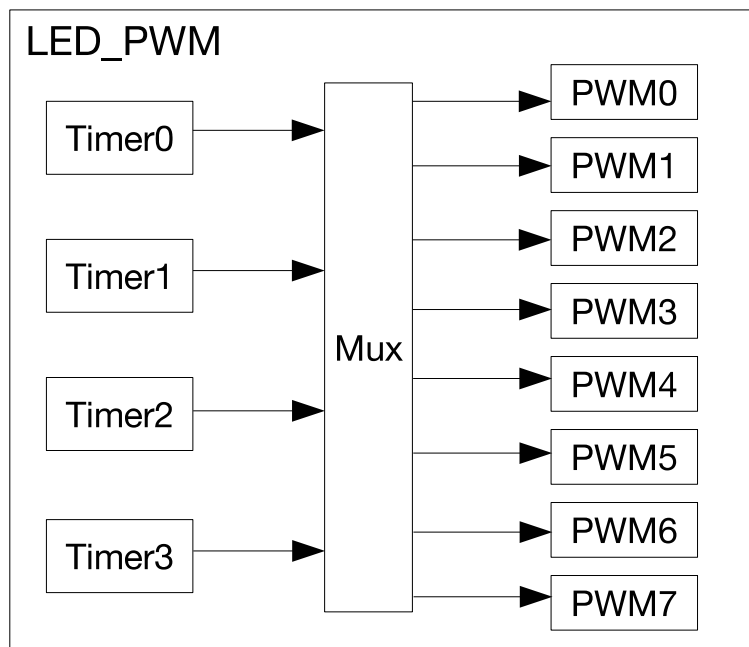
Figure 11-1. LED_PWM Architecture
