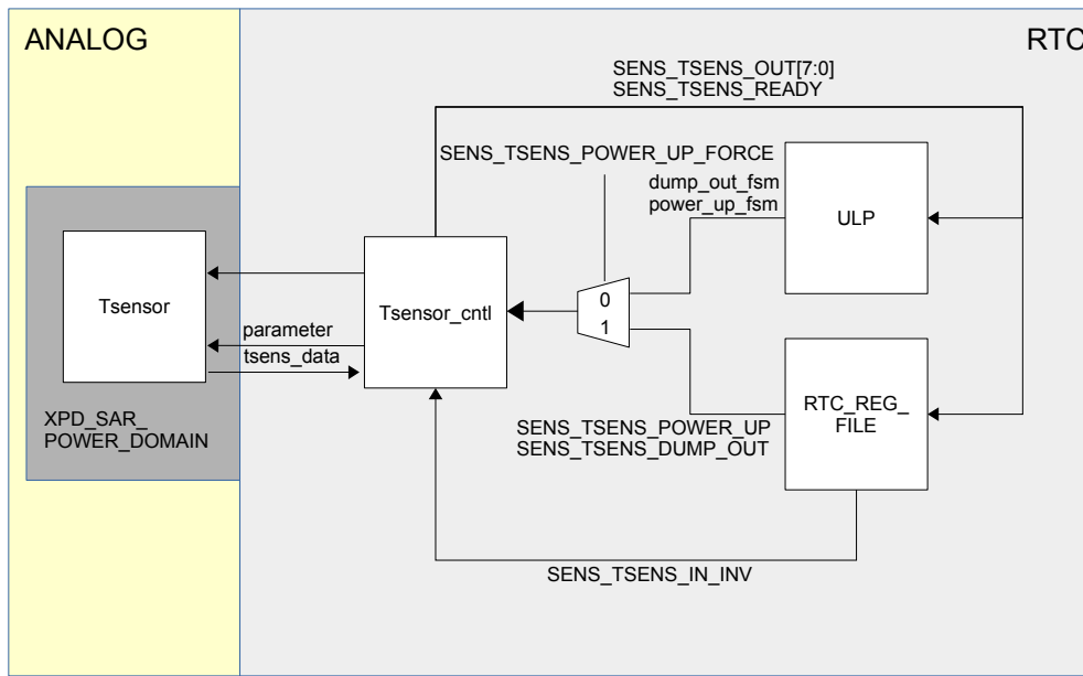
Figure 30-7. Structure of Temperature Sensor
