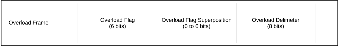
Figure 21-13. The Bit Fields of an Overload Frame
