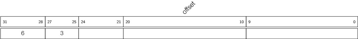
Figure 31-11. Instruction Type - Offset in Automatic Storage Mode (ST-OFFSET)
