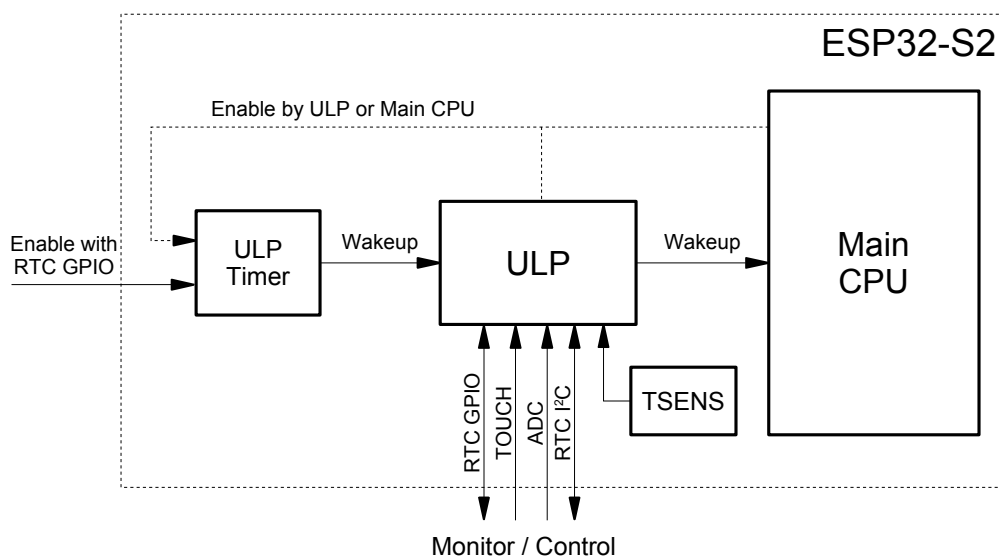
Figure 31-1. ULP Coprocessor Overview
