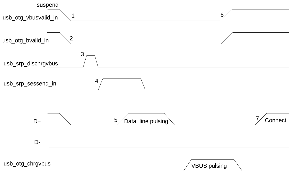
Figure 20-8. B-Device SRP
