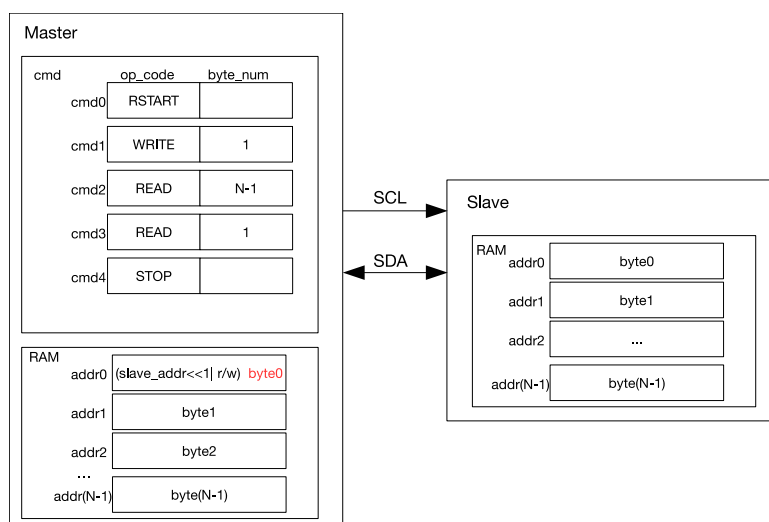
Figure 19-9. An I2C Master Reading an I2C Slave with a 7-bit Address
