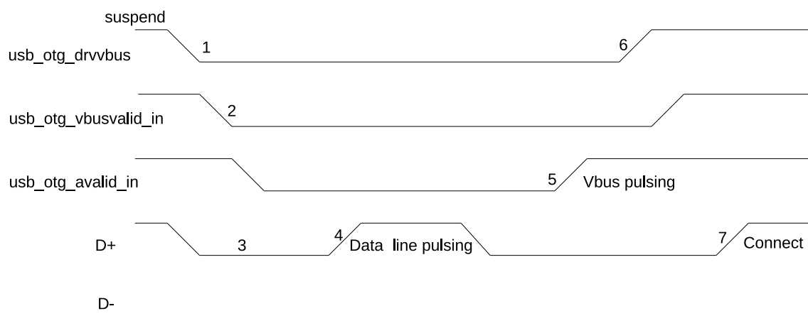
Figure 20-7. A-Device SRP
