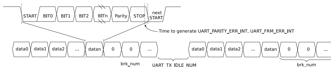
Figure 10-36. Structure of UART Data Frame
