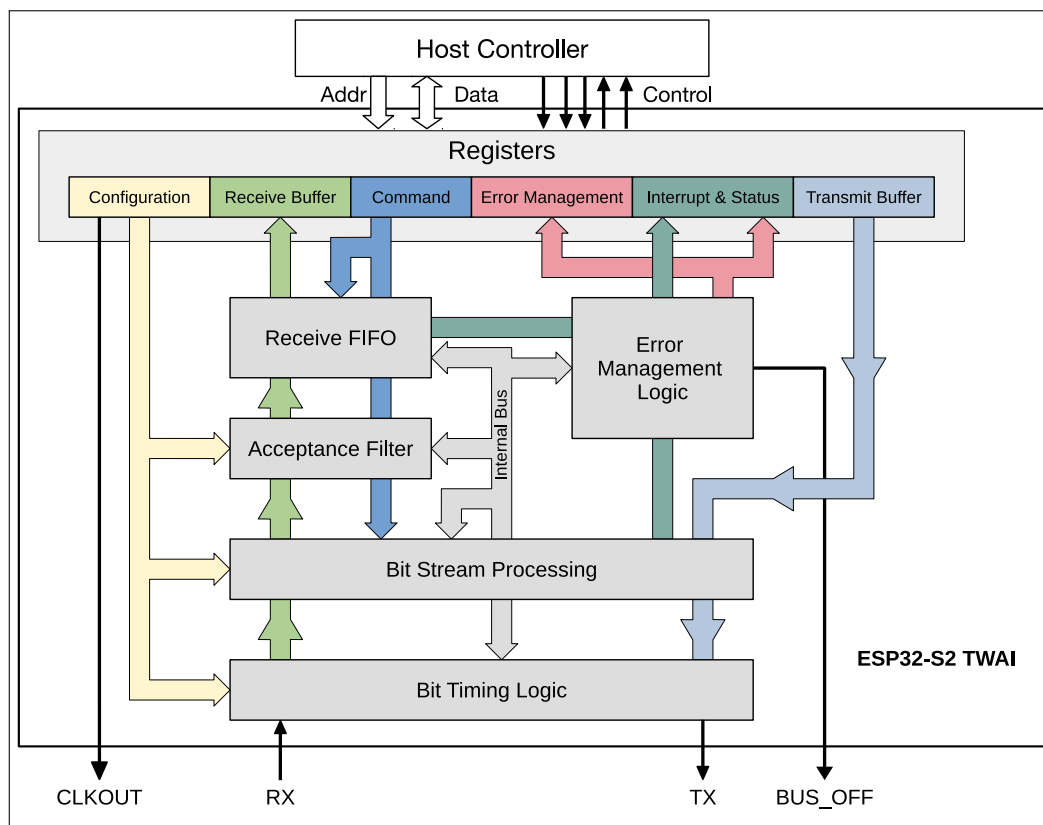
Figure 21-16. TWAI Overview Diagram
