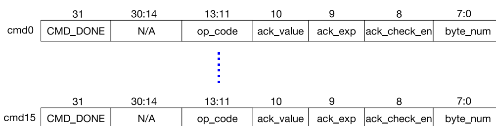
Figure 19-3. Structure of I2C Command Register
