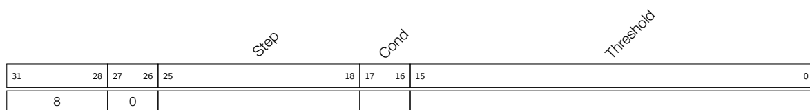
Figure 31-16. Instruction Type - JUMPR
