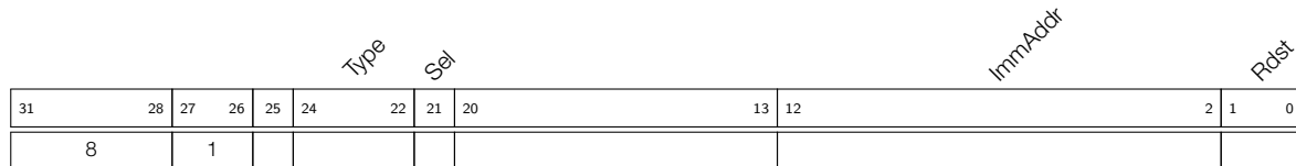
Figure 31-15. Instruction Type- JUMP
