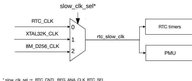
Figure 32-4. Low-Power Slow Clocks for RTC Power Domains
