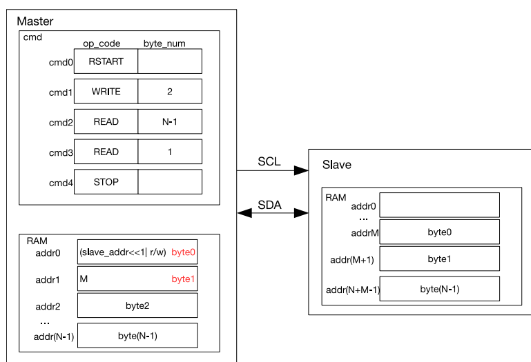
Figure 19-11. An I2C Master Reading N Bytes of Data from addrM of an I2C Slave with a 7-bit Address
