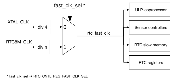
Figure 32-3. Low-Power Fast Clocks for RTC Power Domains
