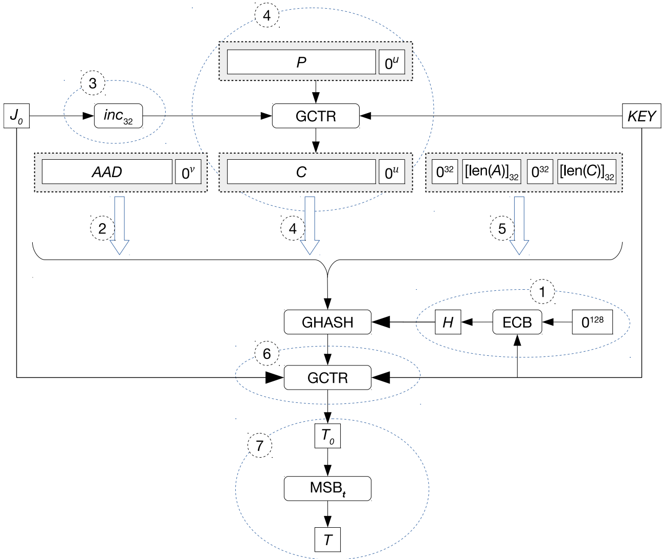
Figure 22-22. GCM Encryption Process
