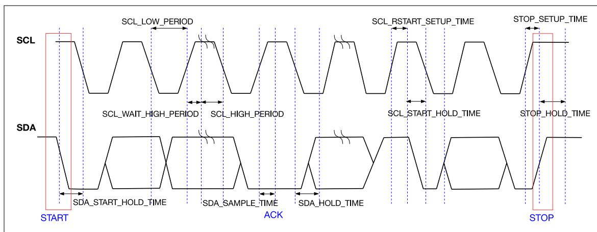
Figure 19-4. I2C Timing Diagram
