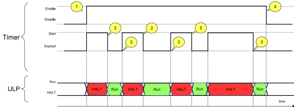
Figure 31-4. Sample of a ULP Operation Sequence
