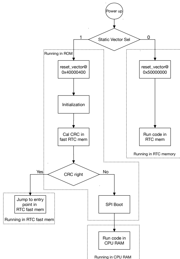
Figure 32-11. ESP32-S2 Boot Flow
