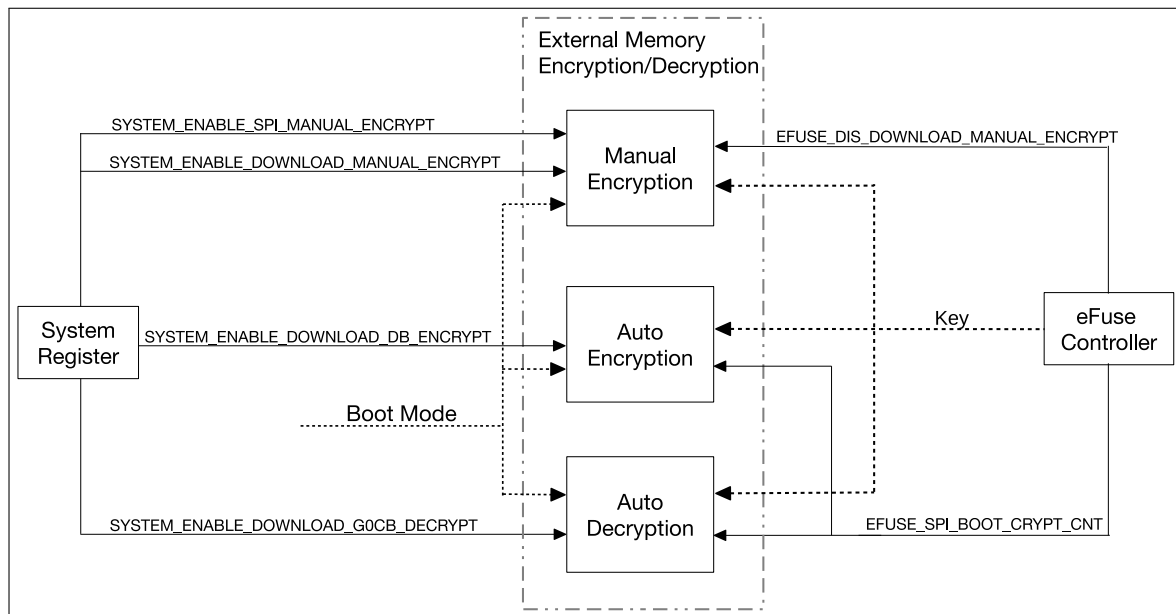
Figure 26-1. Architecture of the External Memory Encryption and Decryption Module
