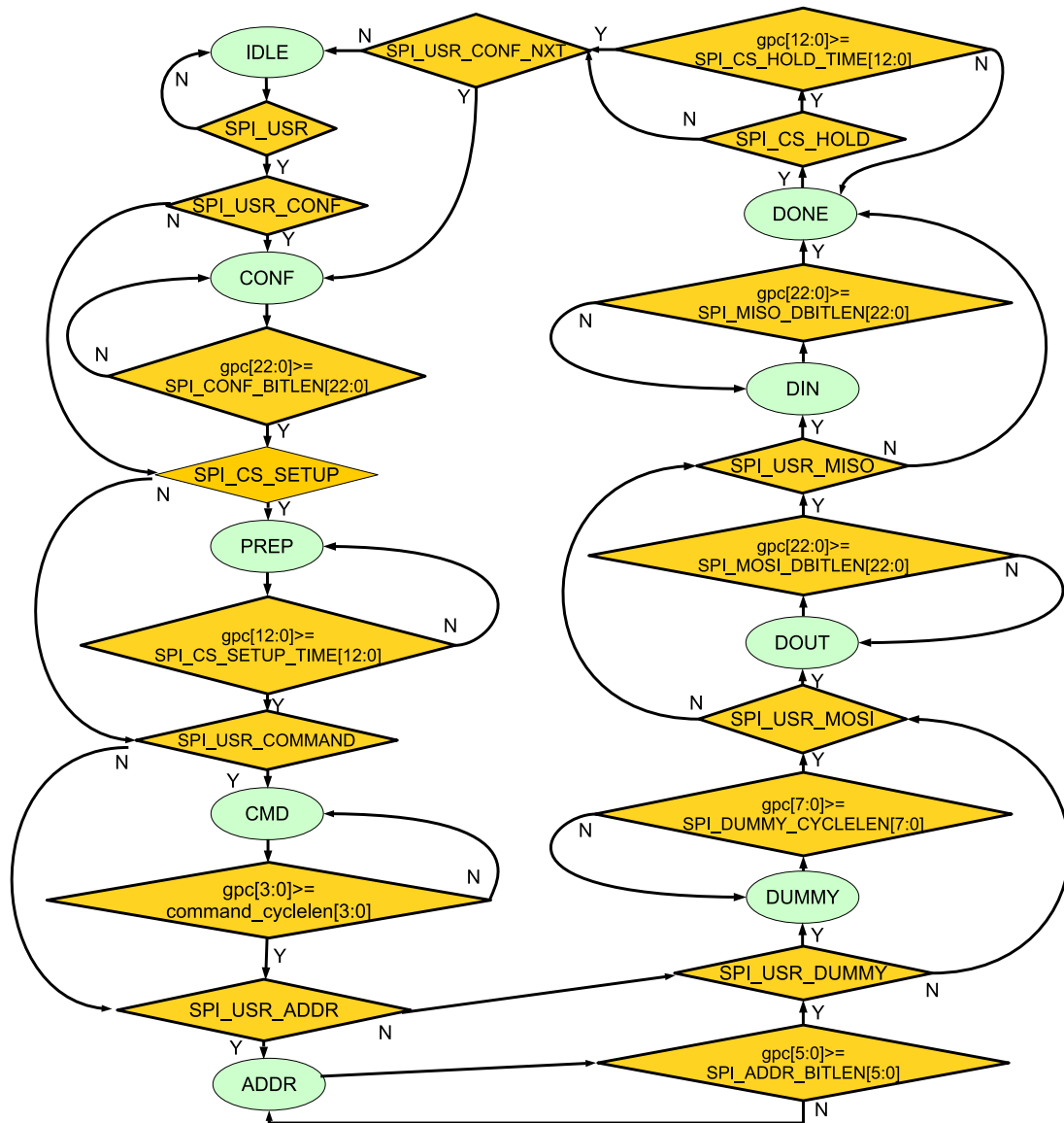
Figure 8-3. GP-SPI2 State Flow in Master Mode
