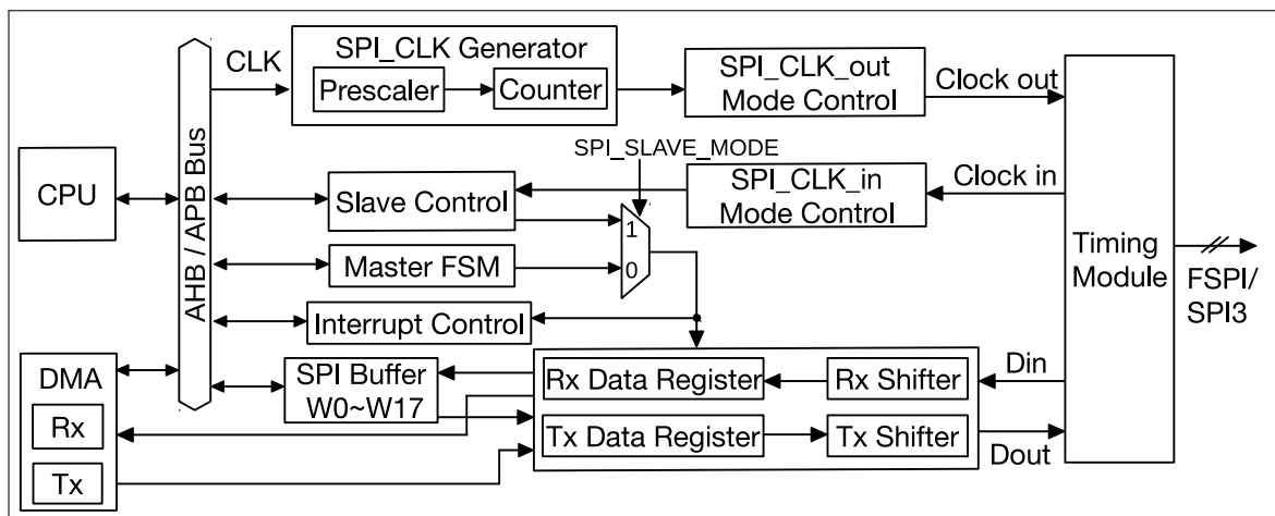
Figure 8-2. GP-SPI2/GP-SPI3 Block Diagram
