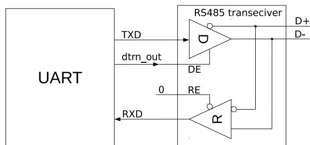
Figure 10-38. Driver Control Diagram in RS485 Mode
