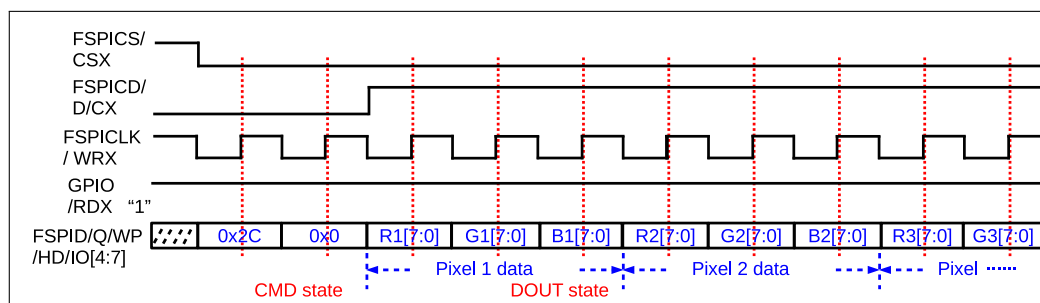
Figure 8-8. Write Command Sequence to an 8-bit LCD Driver
