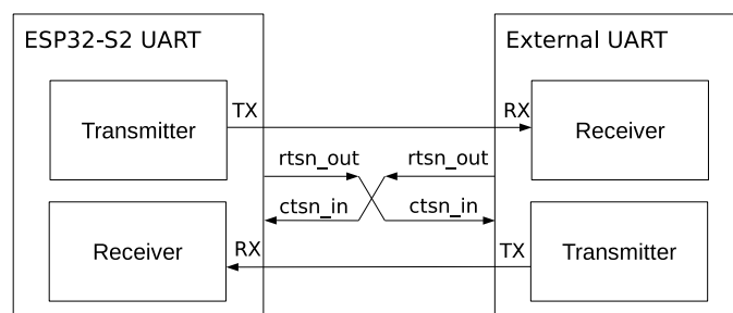
Figure 10-42. Connection between Hardware Flow Control Signals
