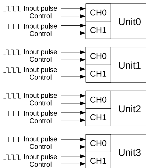
Figure 13-1. PCNT Block Diagram
