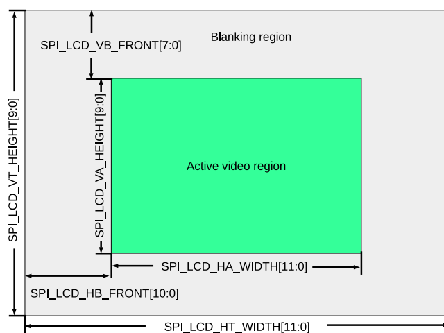
Figure 8-10. Video Frame Structure in Parallel RGB 8-bit LCD Mode
