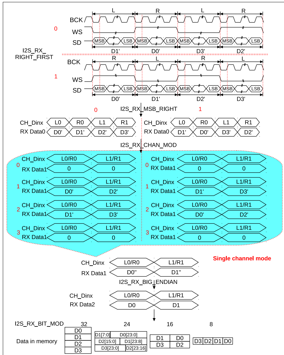
Figure 9-27. ESP32-S2 I2S RX Data When I2S_RX_DMA_EQUAL = 1
