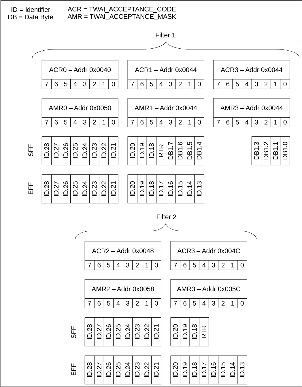
Figure 21-19. Dual Filter Mode
