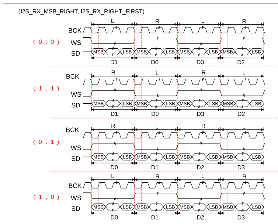
Figure 9-26. I2S RX Data When I2S_RX_DMA_EQUAL = 0
