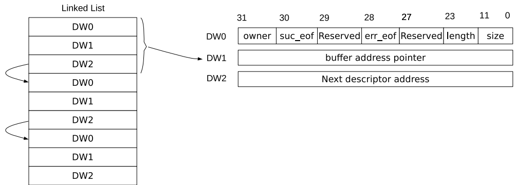
Figure 7-3. Structure of a Linked List
