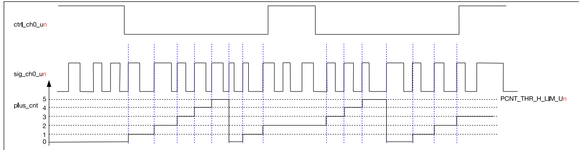
Figure 13-3. Channel 0 Up Counting Diagram
