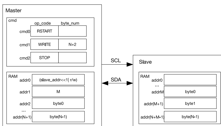
Figure 19-7. An I2C Master Writing Address M in the RAM to an I2C Slave with a 7-bit Address
