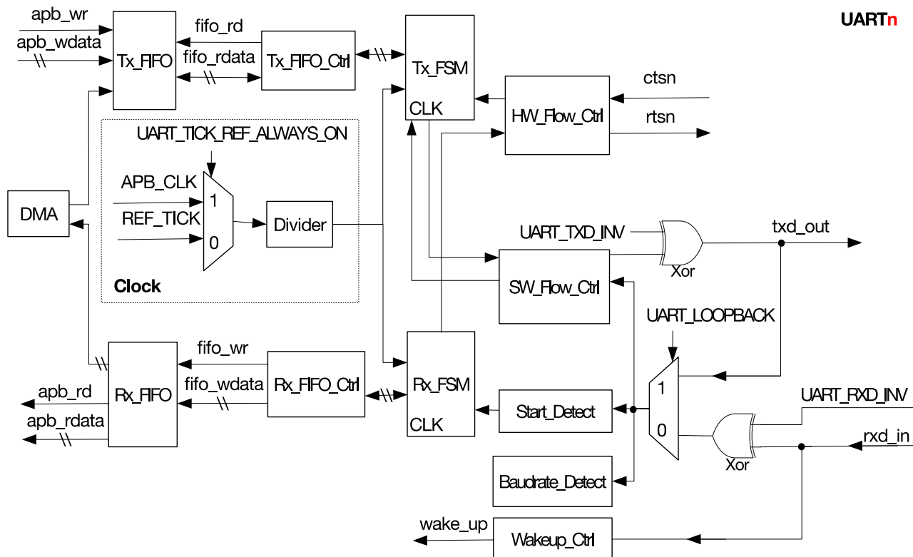
Figure 10-32. UART Structure
