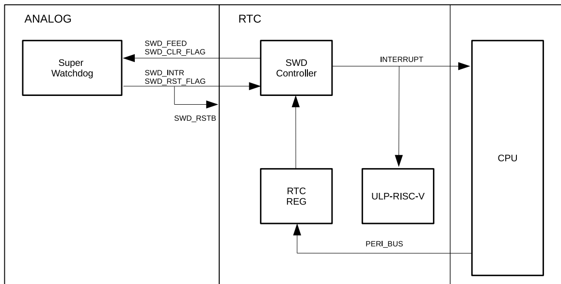
Figure 15-1. Super Watchdog Controller Structure
