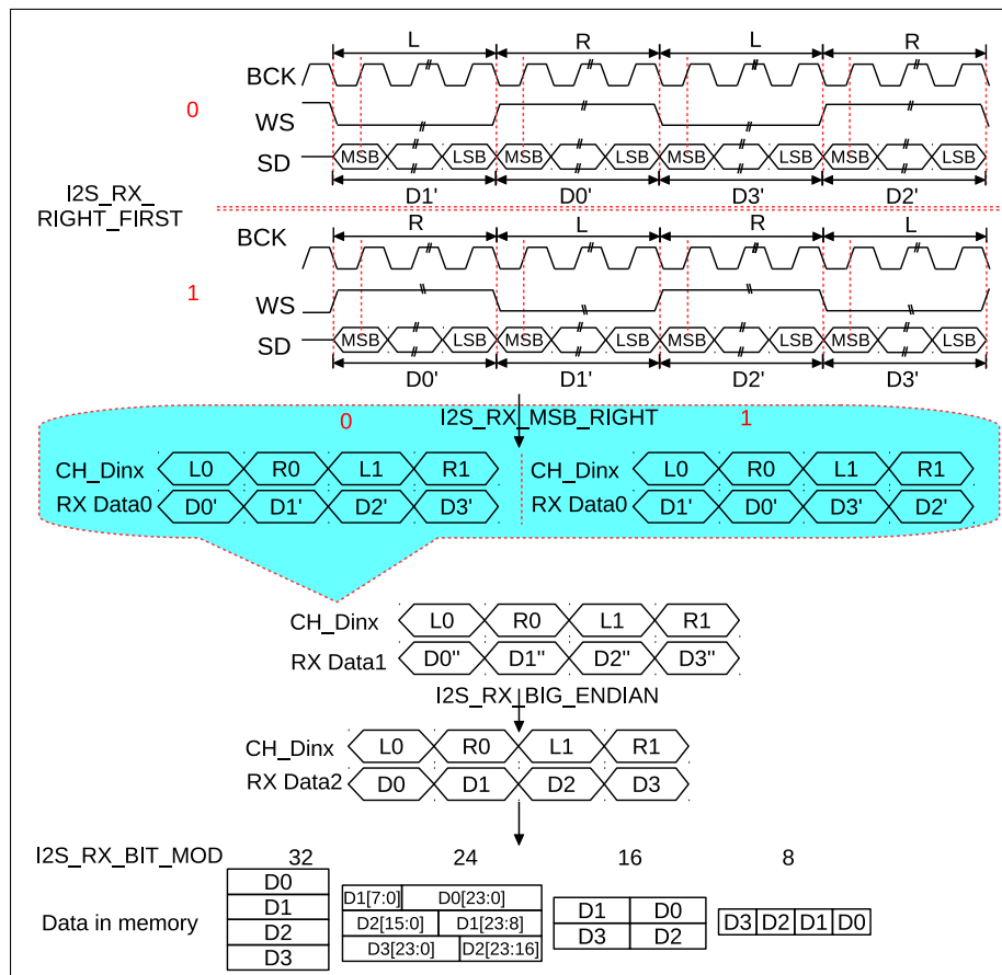
Figure 9-25. I2S RX Data When I2S_RX_DMA_EQUAL = 0
