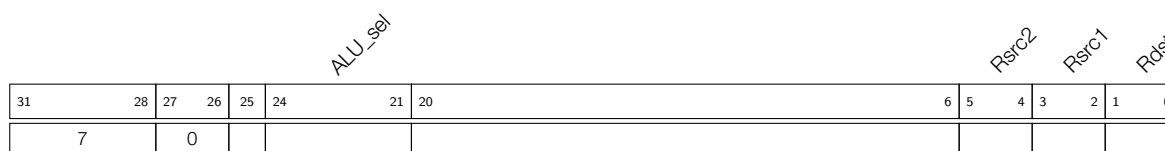
Figure 31-7. Instruction Type — ALU for Operations Among Registers
