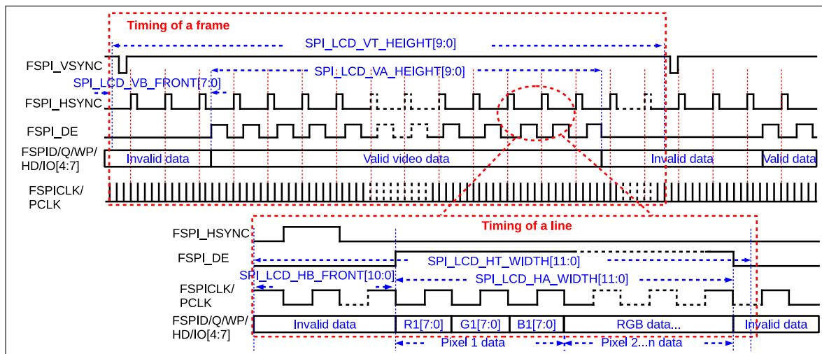
Figure 8-11. Timing Sequence in Parallel RGB 8-bit LCD Mode
