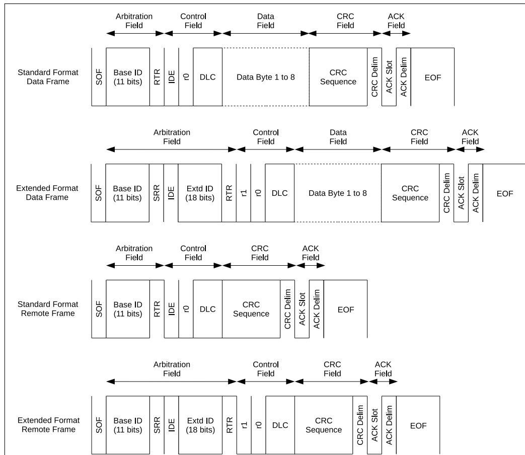
Figure 21-11. The bit fields of Data Frames and Remote Frames
