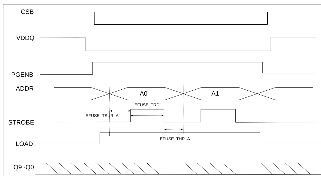
Figure 18-3. Timing Diagram for Reading eFuse
