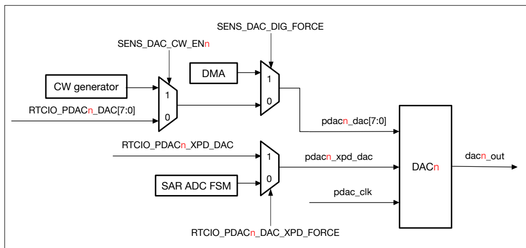
Figure 30-5. Diagram of DAC Function
