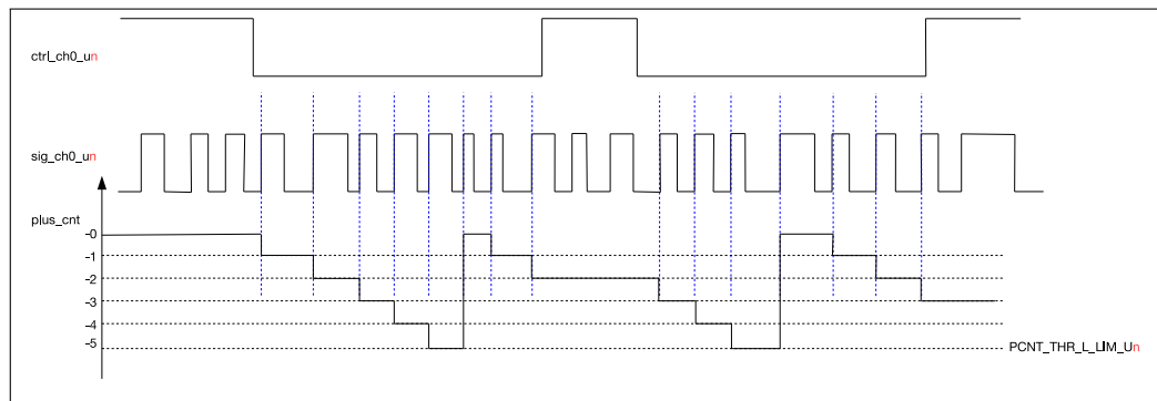
Figure 13-4. Channel 0 Down Counting Diagram
