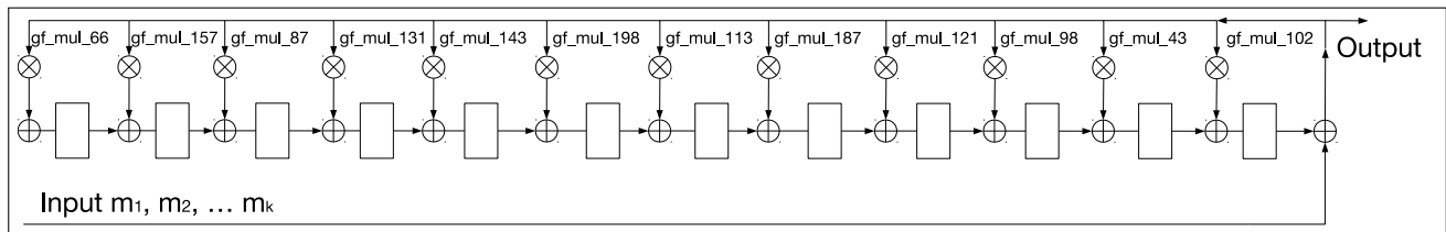
Figure 18-1. Shift Register Circuit
