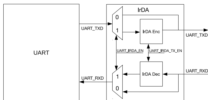
Figure 10-40. IrDA Encoding and Decoding Diagram
