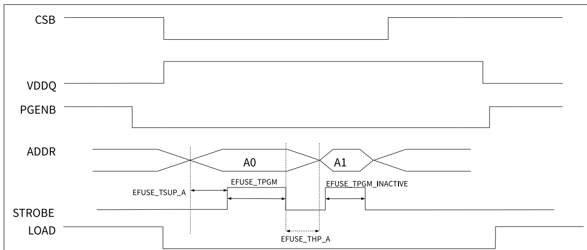
Figure 18-2. eFuse-Programming Timing Diagram
