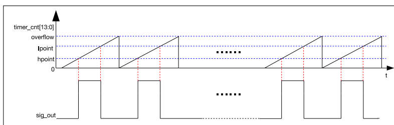
Figure 11-4. LED_PWM Output Signal Diagram
