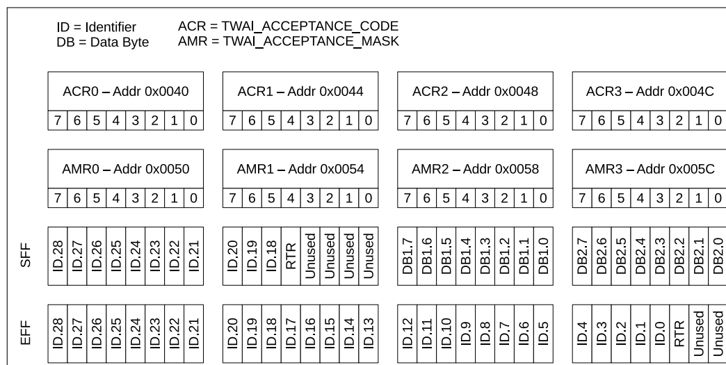
Figure 21-18. Single Filter Mode
