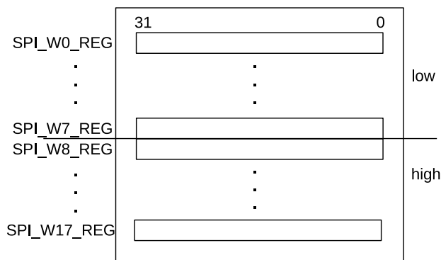
Figure 8-14. Data Buffer Used in CPU-Controlled Mode
