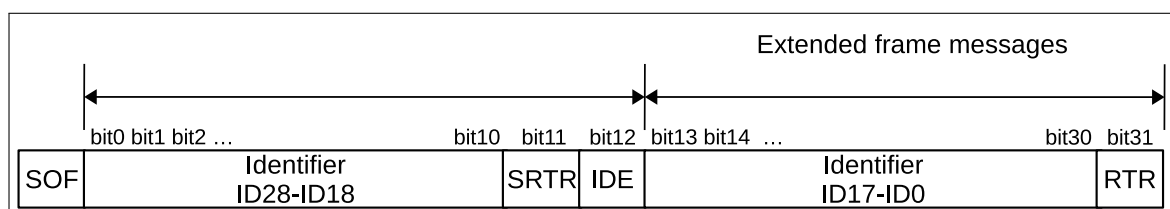
Figure 21-21. Positions of Arbitration Lost Bits
