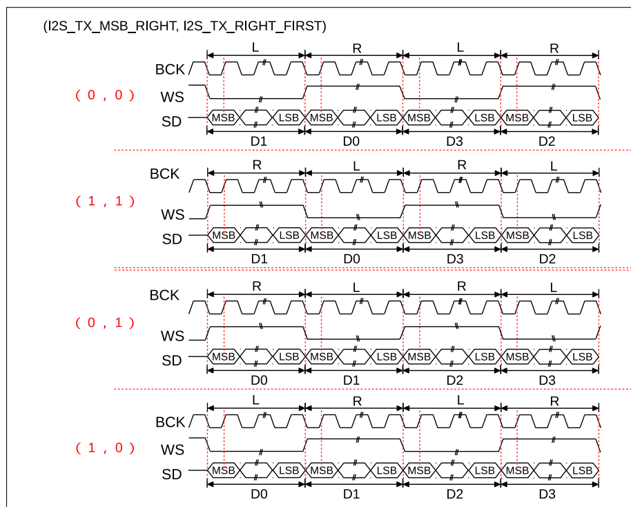
Figure 9-23. I2S Output Format When I2S_TX_CHAN_MOD[2:0] = 0 and I2S_TX_DMA_EQUAL = 0
