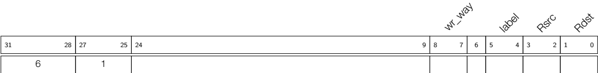
Figure 31-12. Instruction Type - Data Storage in Automatic Storage Mode (ST-AUTO-DATA)
