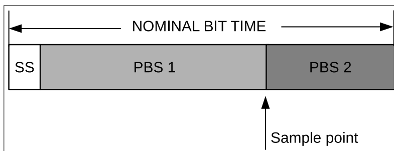
Figure 21-15. Layout of a Bit
