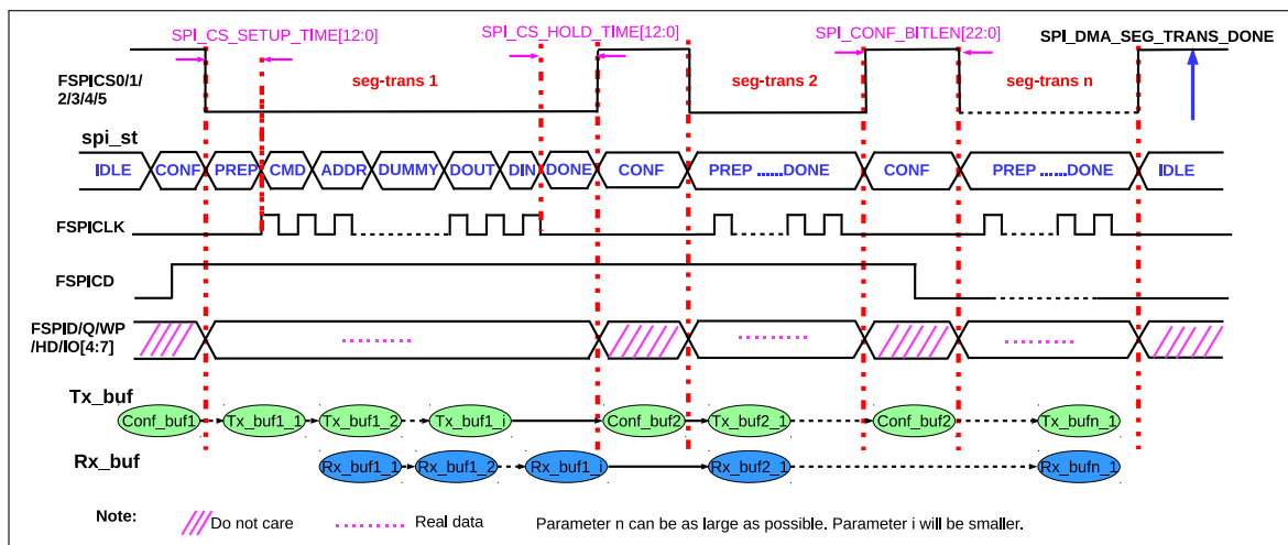
Figure 8-9. Segmented-Configure-Transfer in DMA Controlled Master Mode
