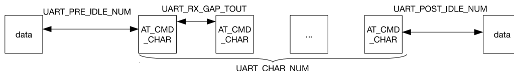
Figure 10-37. AT_CMD Character Structure
