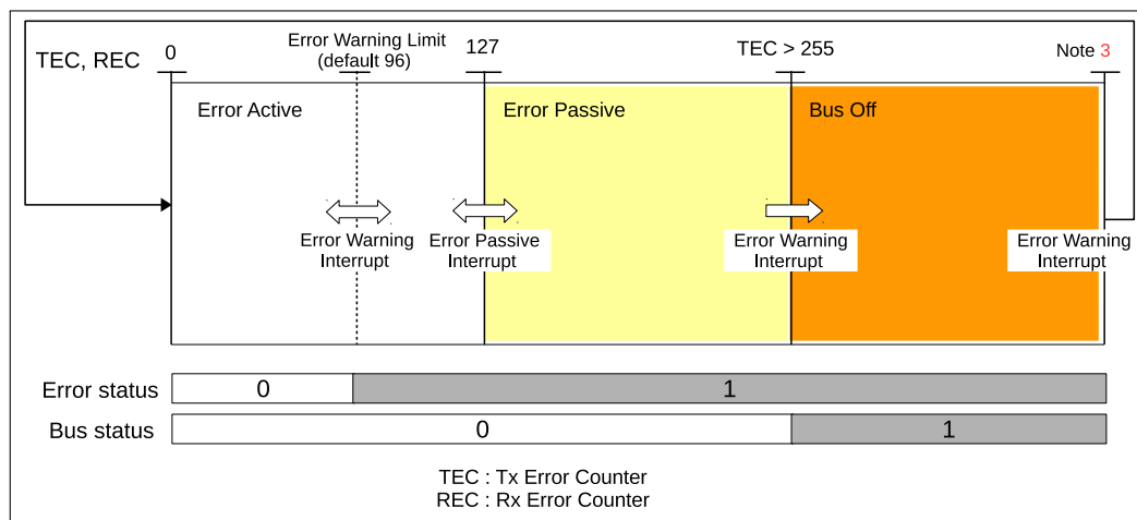
Figure 21-20. Error State Transition
