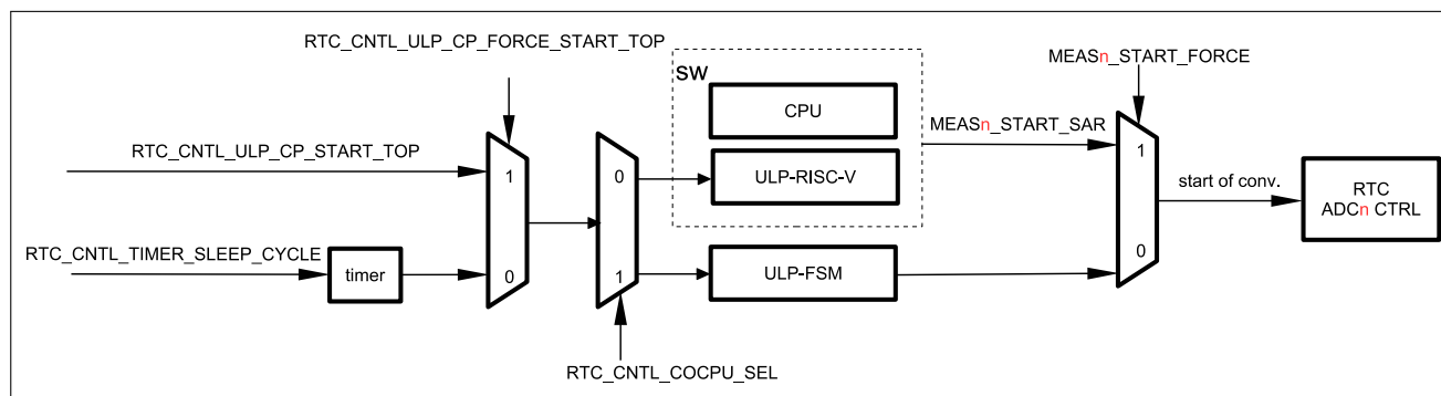
Figure 30-3. RTC SAR ADC Outline
