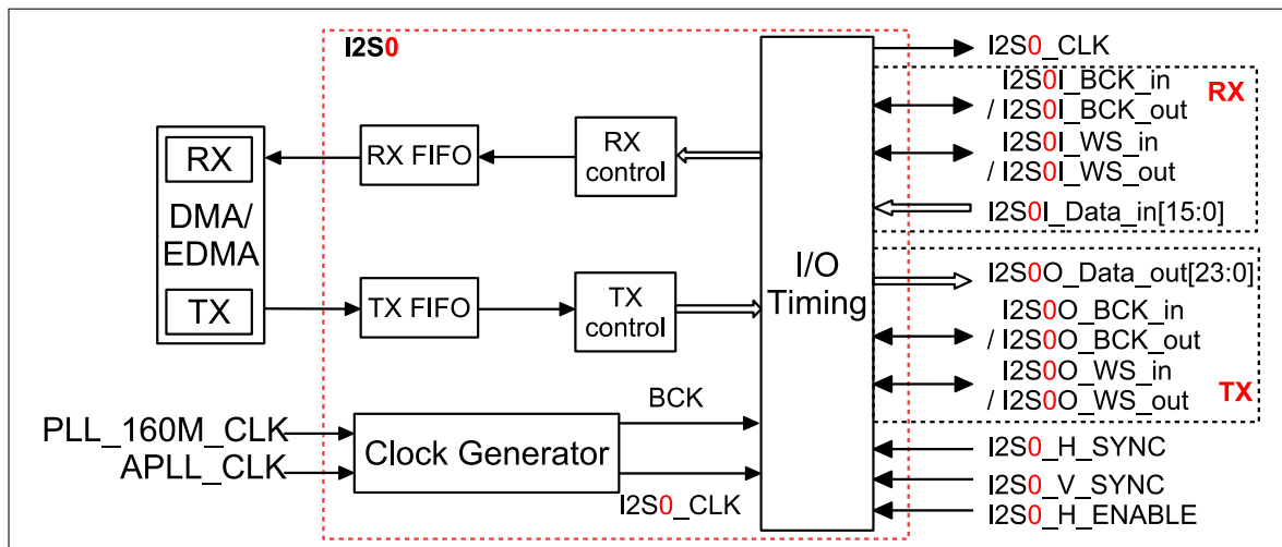
Figure 9-17. ESP32-S2 I2S System Diagram
