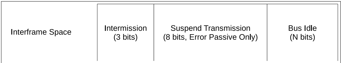
Figure 21-14. The Fields within an Interframe Space
