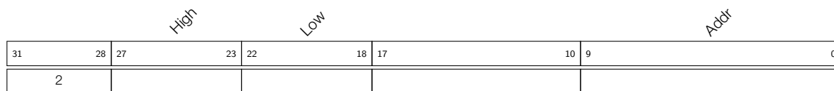
Figure 31-23. Instruction Type - REG_RD
