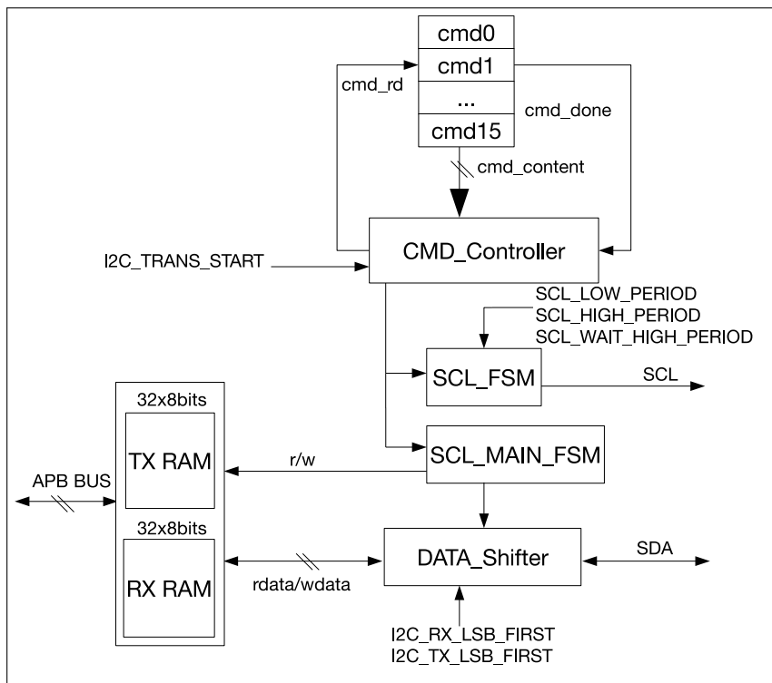
Figure 19-1. I2C Master Architecture
