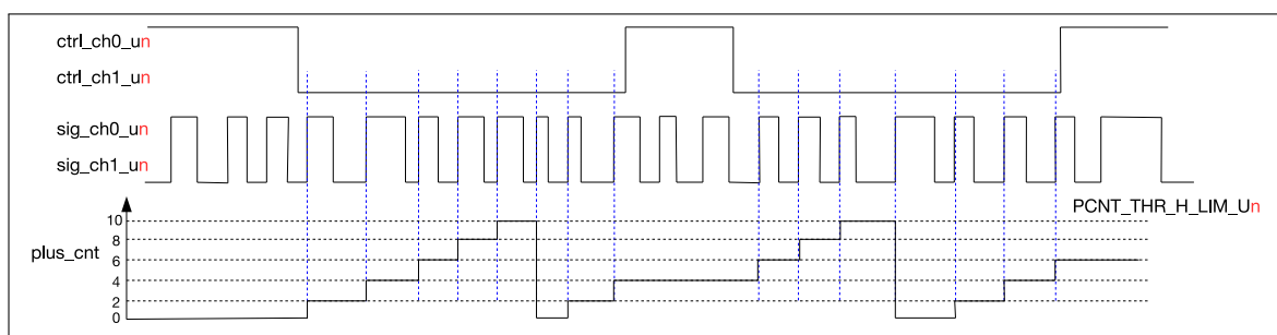
Figure 13-5. Two Channels Up Counting Diagram
