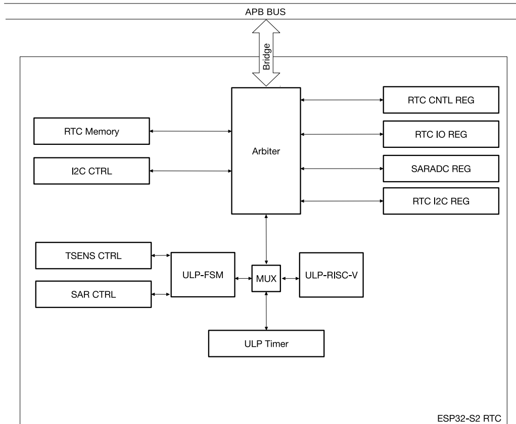
Figure 31-2. ULP Coprocessor Diagram
