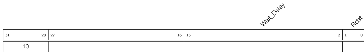
Figure 31-21. Instruction Type - TSENS
