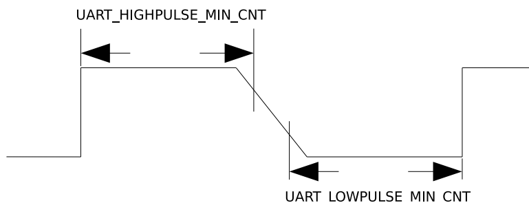
Figure 10-35. The Timing Diagram of Weak UART Signals Along Falling Edges
