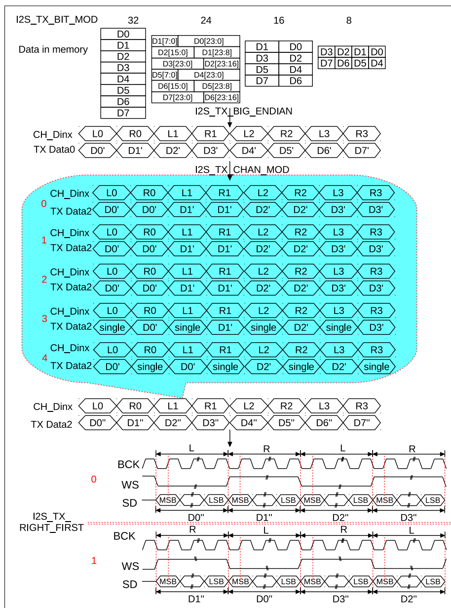
Figure 9-24. I2S TX Data When I2S_TX_DMA_EQUAL = 1
