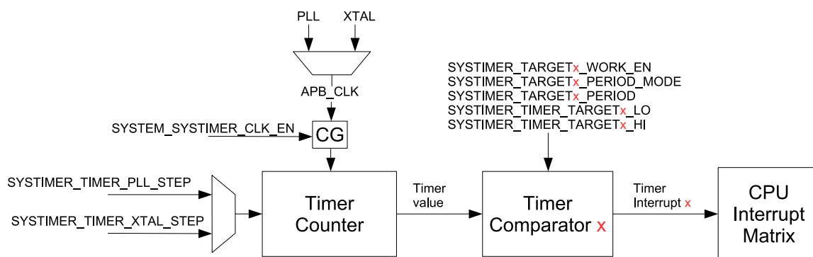
Figure 17-1. System Timer Structure
