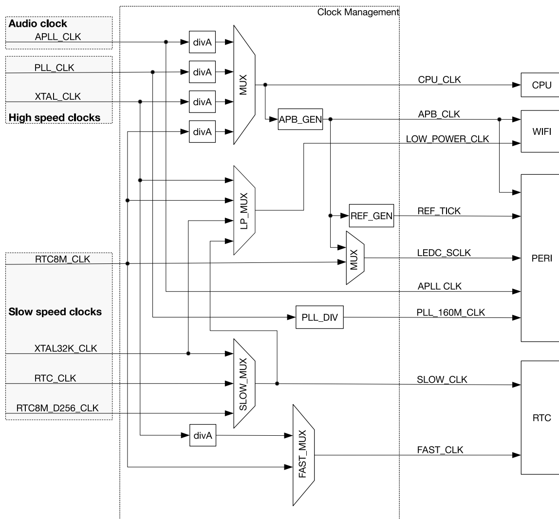
Figure 2-2. System Clock
