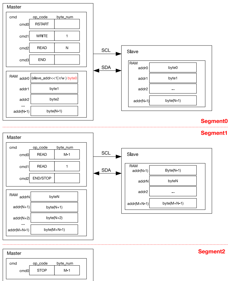
Figure 19-12. An I2C Master Reading an I2C Slave with a 7-bit Address in Segments
