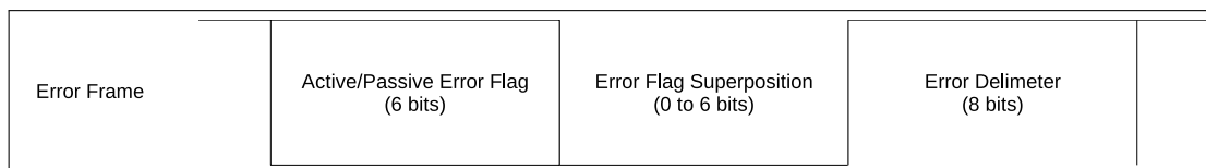
Figure 21-12. Various Fields of an Error Frame
