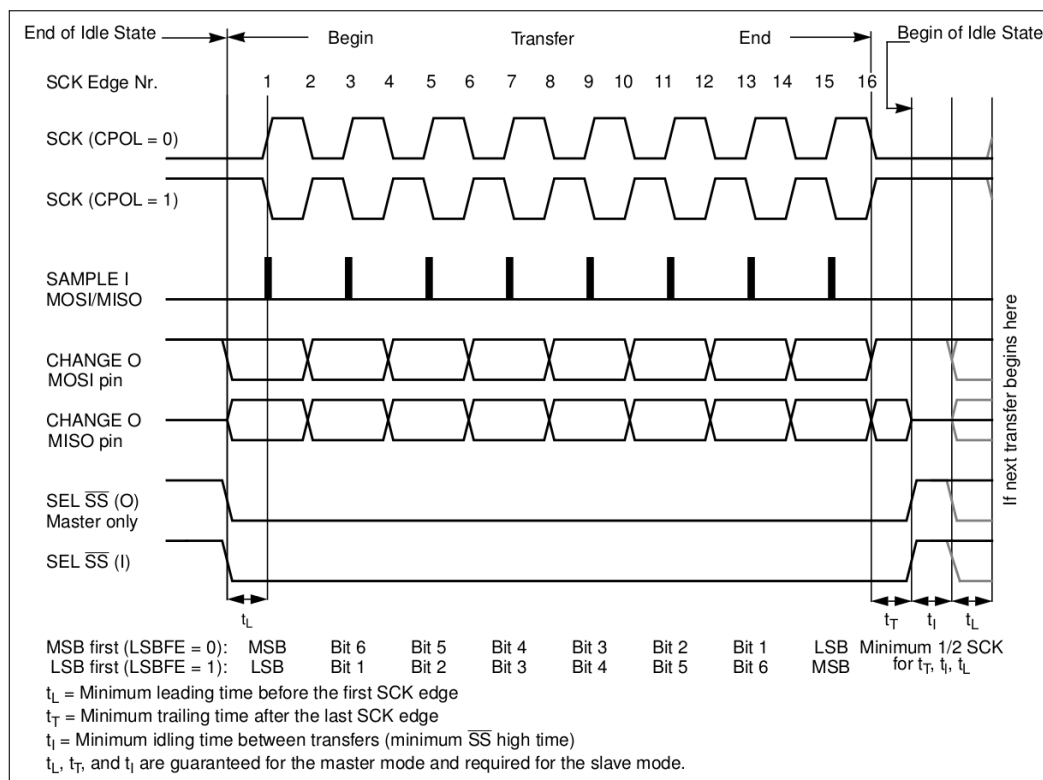
Figure 8-15. SPI CLK Mode 0 or 2
