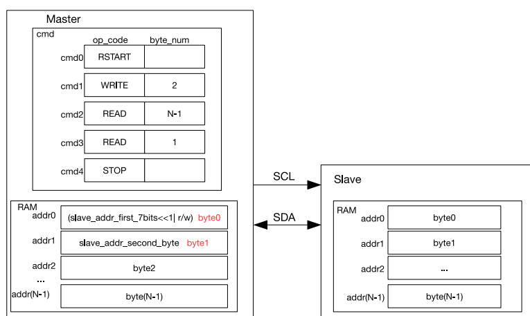
Figure 19-10. An I2C Master Reading an I2C Slave with a 10-bit Address
