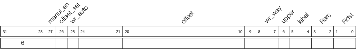
Figure 31-10. Instruction Type - ST
