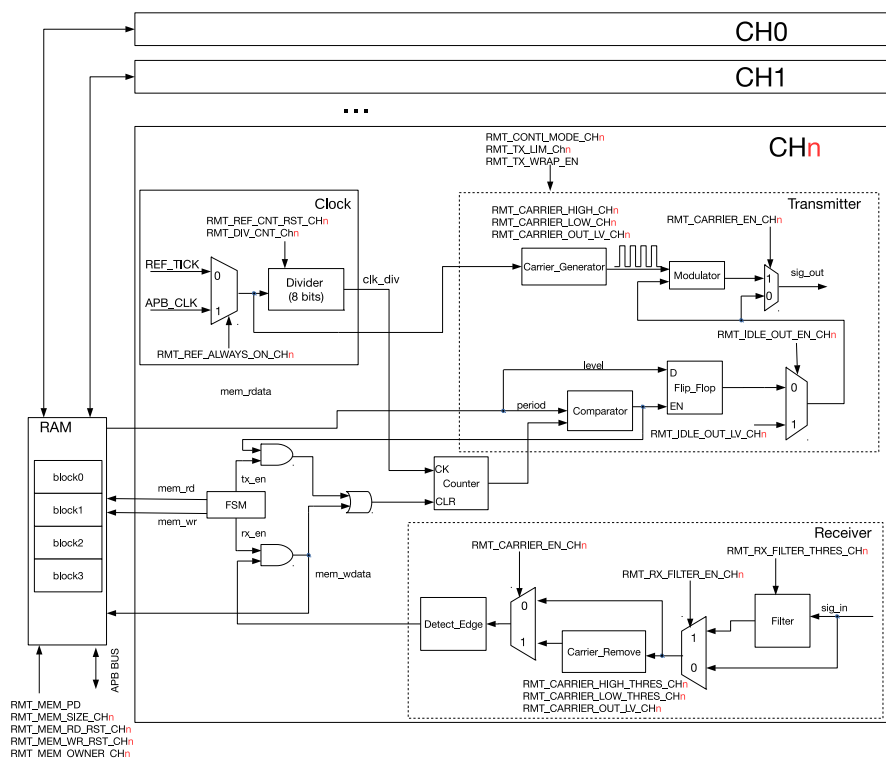
Figure 12-1. RMT Architecture
