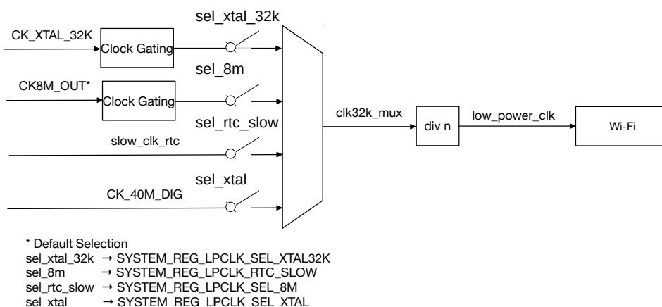
Figure 32-5. Low-Power Clocks for RTC Fast Memory and Slow Memory
