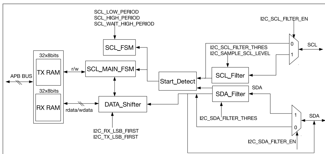
Figure 19-2. I2C Slave Architecture
