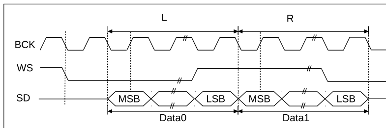
Figure 9-18. Philips Standard
