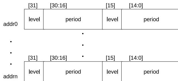
Figure 12-2. Format of Pulse Code in RAM
