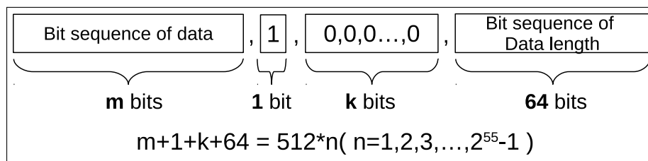
Figure 29-1. HMAC SHA-256 Padding Diagram
