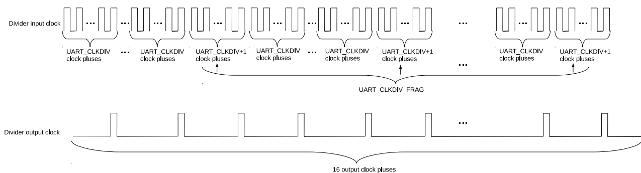
Figure 10-34. UART Controllers Division
