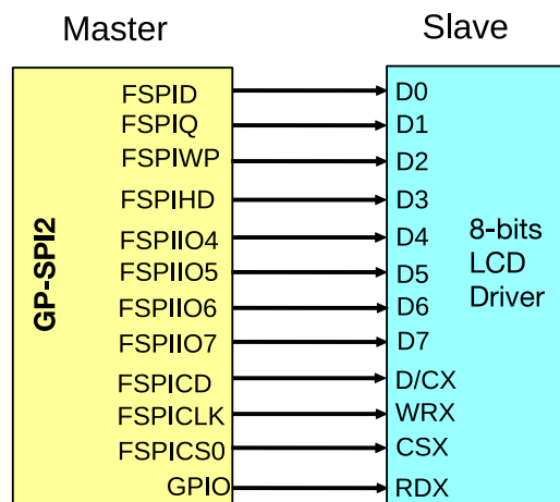
Figure 8-7. Connection of GP-SPI2 to 8-bit LCD Driver
