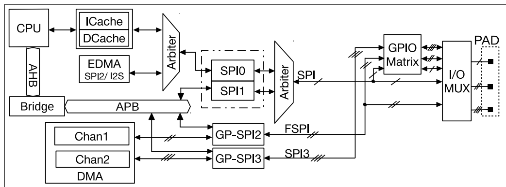
Figure 8-1. SPI Block Diagram
