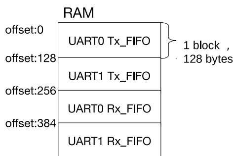
Figure 10-33. UART Controllers Sharing RAM
