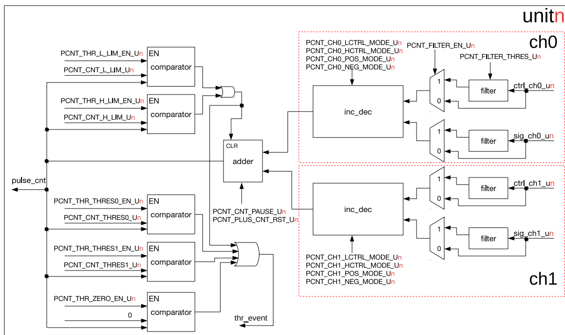
Figure 13-2. PCNT Unit Architecture
