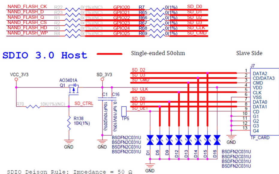
Fig. 7: ESP32-S31-Korvo-1 V1.1 - microSD card function (click to enlarge)
