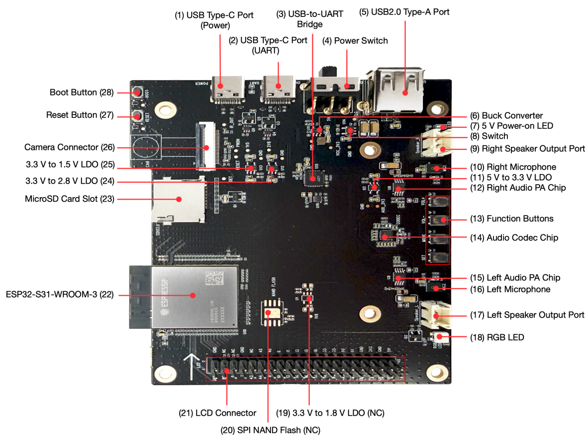
Fig. 2: ESP32-S31-Korvo-1 V1.1 (click to enlarge)
