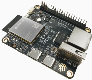
ESP32-S31-Function-CoreBoard-1
