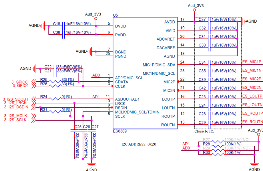
Fig. 6: ESP32-S31-Korvo-1 V1.1 - ES8389 audio codec schematic (click to enlarge)
