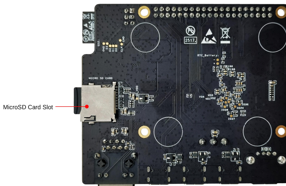
Fig. 3: ESP32-P4-Function-EV-Board - back (click to enlarge)
