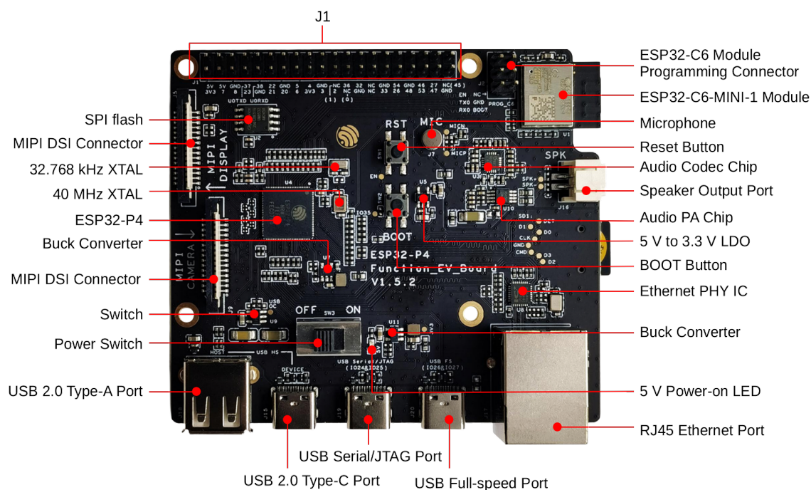
Fig. 2: ESP32-P4-Function-EV-Board - front (click to enlarge)
