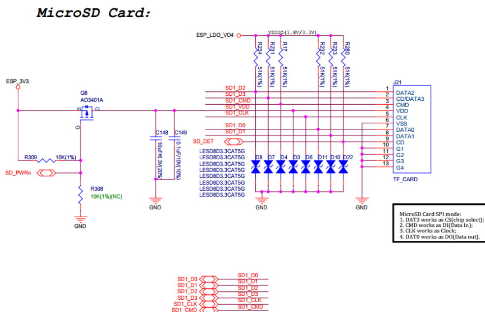
Fig. 12: MicroSD Card Slot Interface Circuit (Click to Enlarge)
