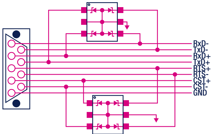
ESDA6V1/14/25xx ESD protection in SOT666/323/23
