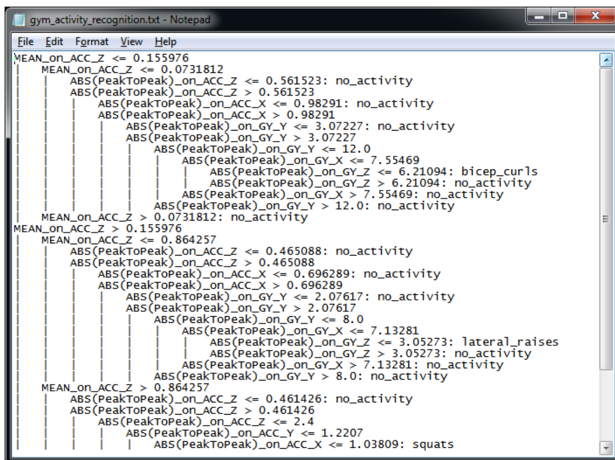
Figure 41. Gym activity recognition decision tree
