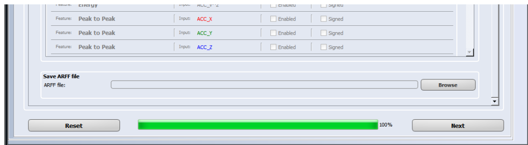
Figure 28. ARFF generation
