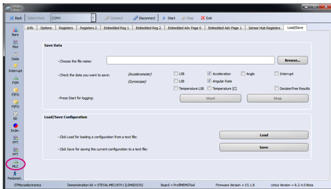
Figure 17. Unico GUI
