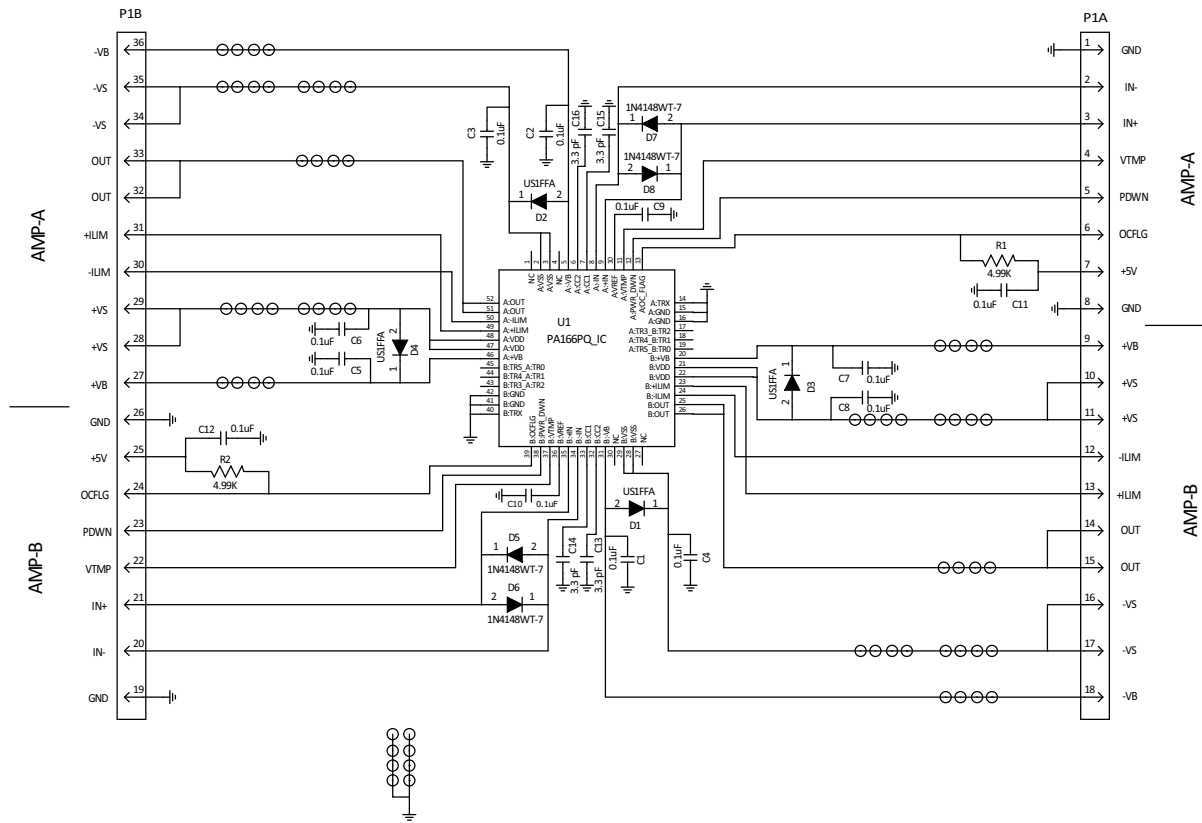
Figure 3: Circuit Diagram (Daughter card PCB (EVAL99))
