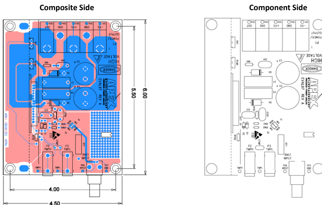
Figure 1: PCB Layout
