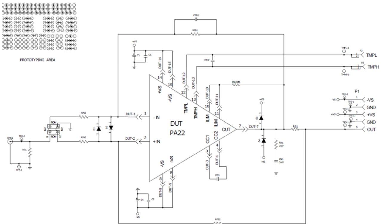
Figure 2: Circuit Diagram
