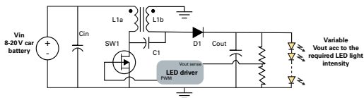
Figure 1. SEPIC circuit
