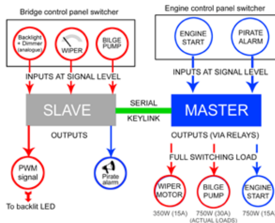
KeyLink: inputs and outputs are connected using a serial half- or full-duplex interface. There can be up to 128 I/O points.
