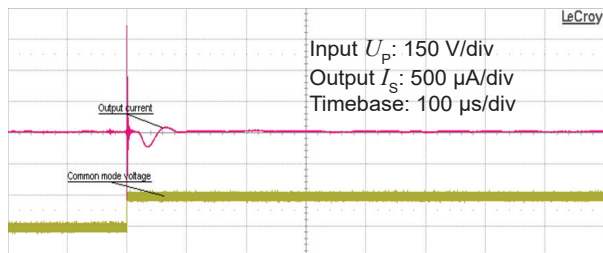
Figure 13: Typical common mode perturbation (150 V step with 6 kV/µs R_M = 100 \Omega )
