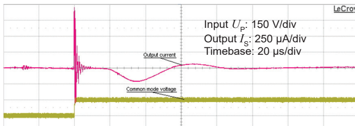
Figure 14: Detail of typical common mode perturbation (150 V step with 6 kV/µs, R_M = 100 \Omega )
