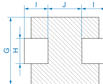
PAD LAYOUT
