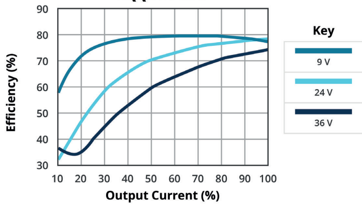
EFFICIENCY VS OUTPUT LOAD DQQ3-24-S3-S
