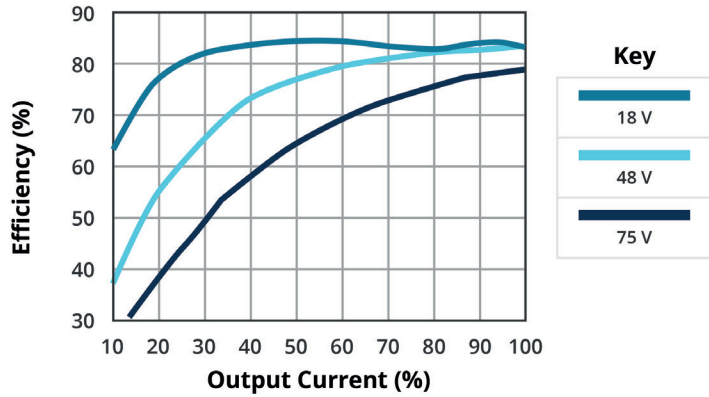
EFFICIENCY VS OUTPUT LOAD DQQ3-48-S15-S
