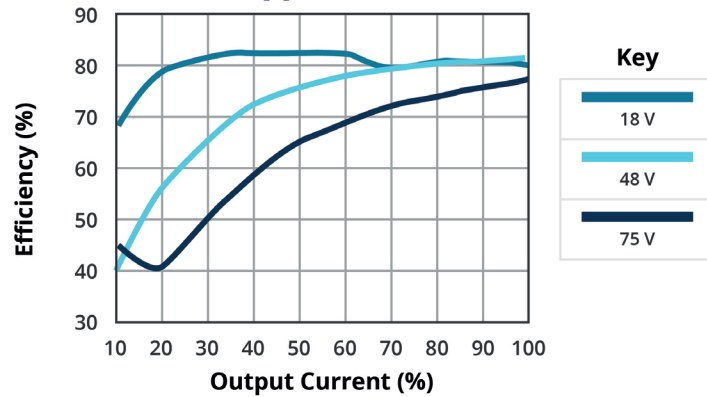
EFFICIENCY VS OUTPUT LOAD DQQ3-48-S5-S
