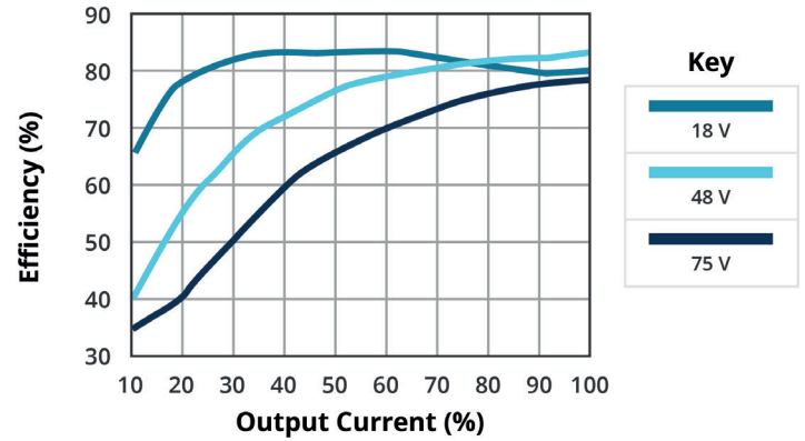
EFFICIENCY VS OUTPUT LOAD DQQ3-48-D5-S
