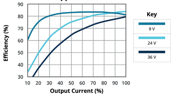
EFFICIENCY VS OUTPUT LOAD DQQ3-24-S15-S
