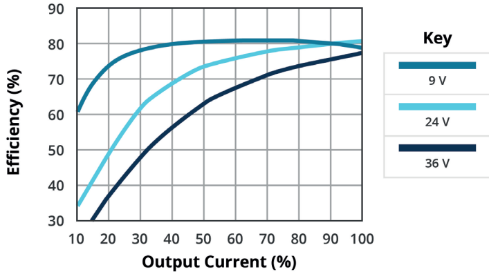
EFFICIENCY VS OUTPUT LOAD DQQ3-24-D5-S
