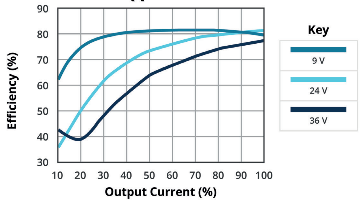
EFFICIENCY VS OUTPUT LOAD DQQ3-24-S5-S
