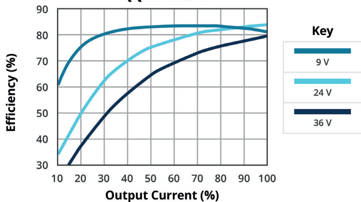
EFFICIENCY VS OUTPUT LOAD DQQ3-24-S12-S
