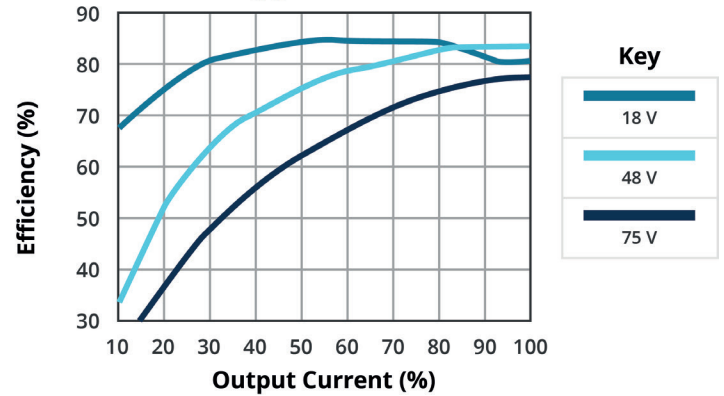
EFFICIENCY VS OUTPUT LOAD DQQ3-48-D15-S
