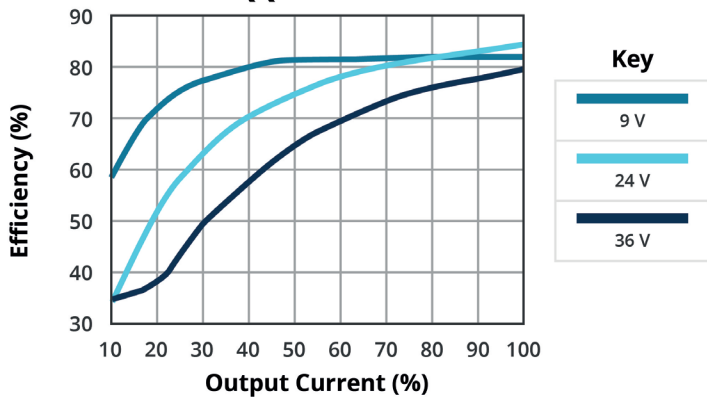
EFFICIENCY VS OUTPUT LOAD DQQ3-24-D15-S
