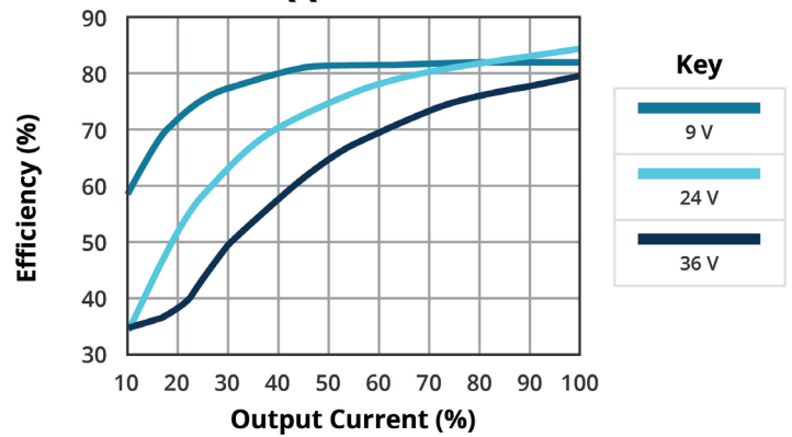
EFFICIENCY VS OUTPUT LOAD DQQ3-48-S3-S
