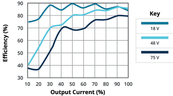
EFFICIENCY VS OUTPUT LOAD DQQ3-48-D12-S
