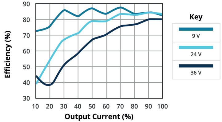
EFFICIENCY VS OUTPUT LOAD DQQ3-24-D12-S
