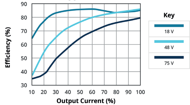
EFFICIENCY VS OUTPUT LOAD DQQ3-48-S12-S
