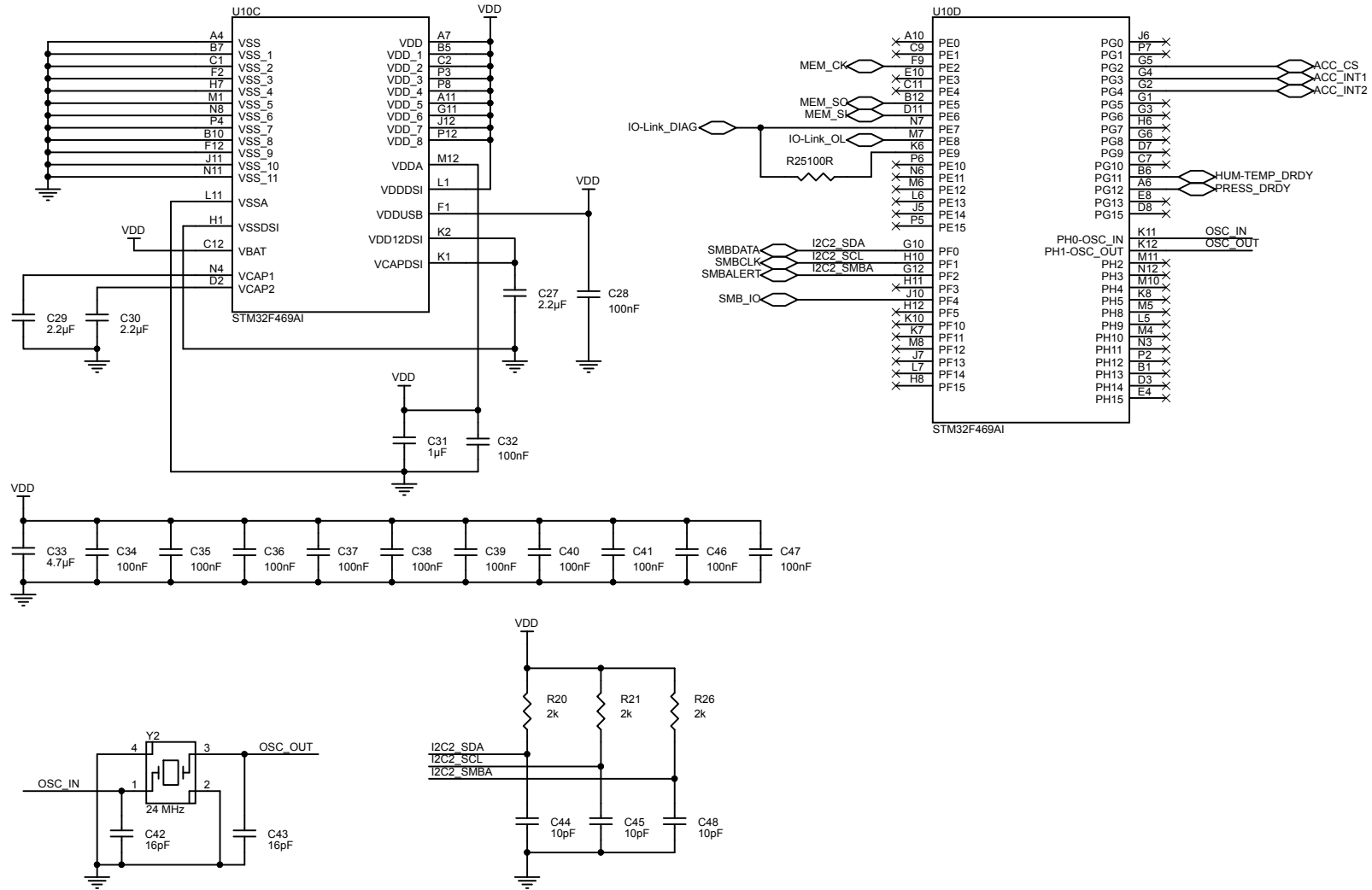
Figure 76. STEVAL-IDP005V2 (main board) circuit schematic - microcontroller (2 of 2)
