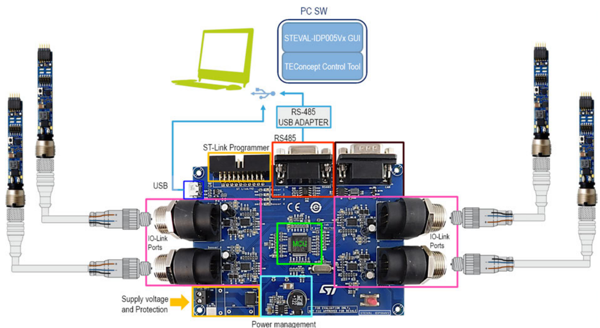
Figure 49. IO-Link System setup with PC communication
