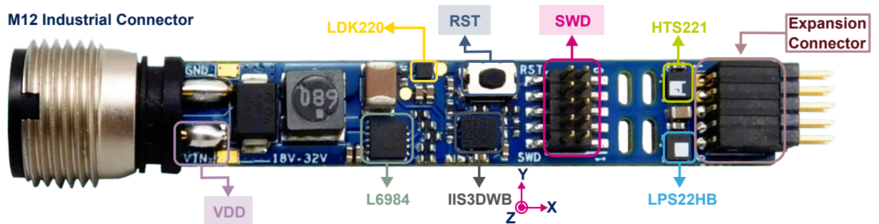
Figure 4. Industrial sensor node - bottom view
