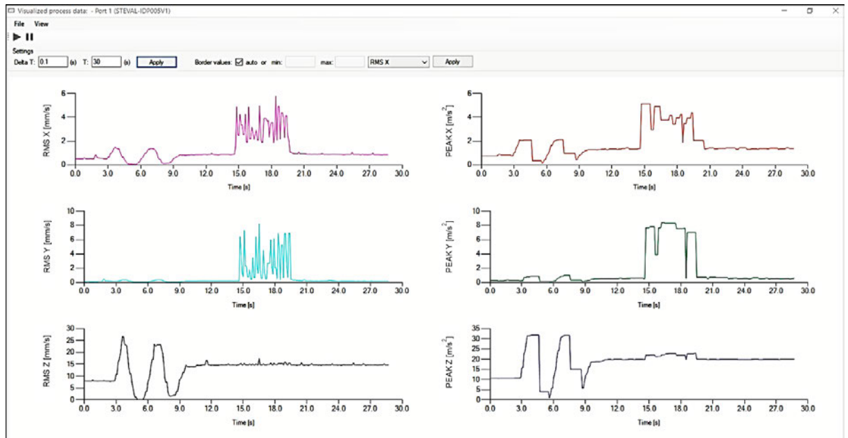
Figure 63. Data plot of Time Domain analysis
