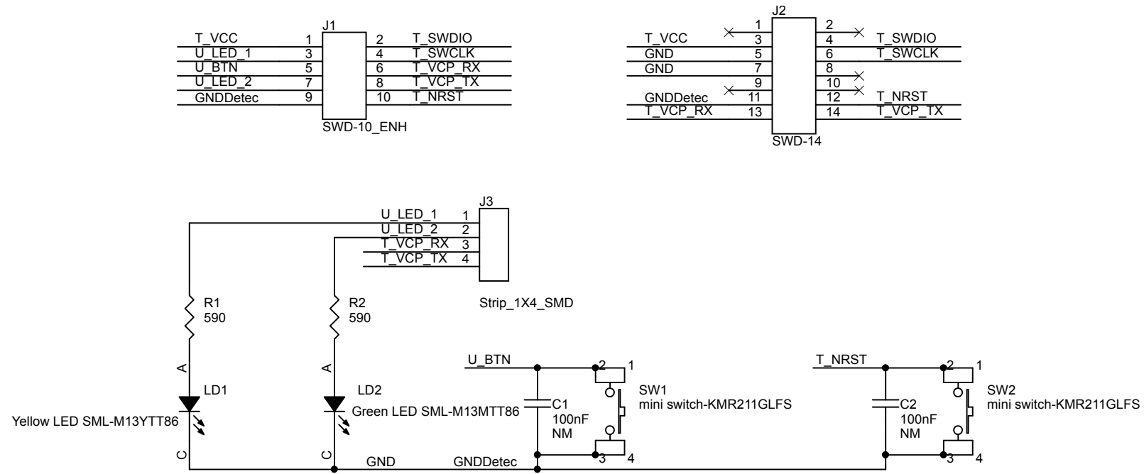
Figure 69. STEVAL-UKI001V2 (adapter board) circuit schematic
