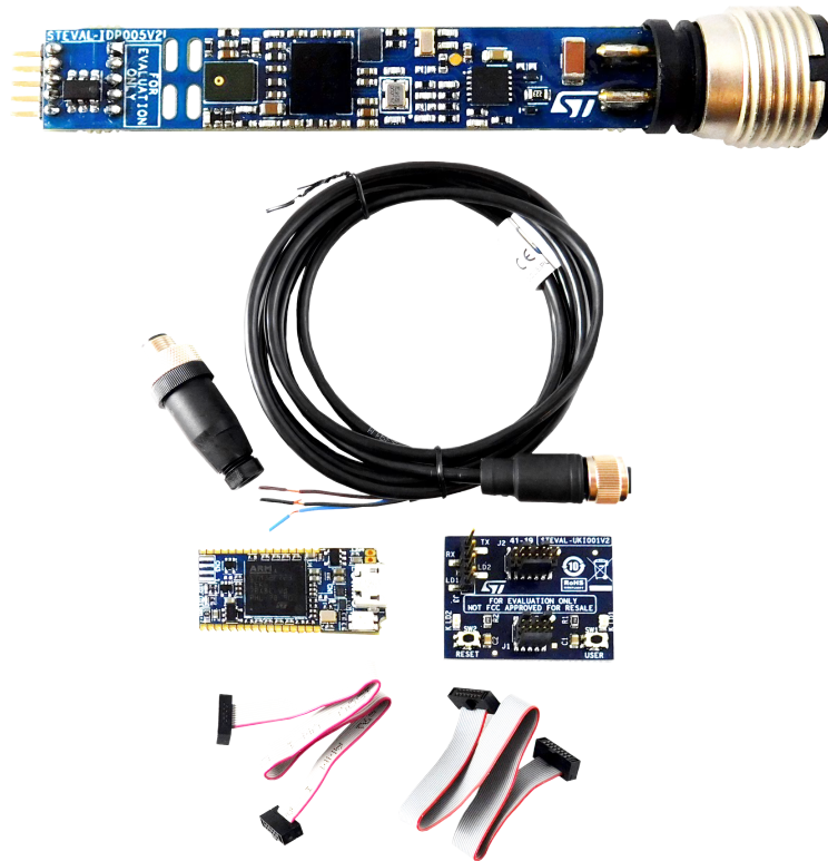
Figure 3. Industrial sensor node - top view
