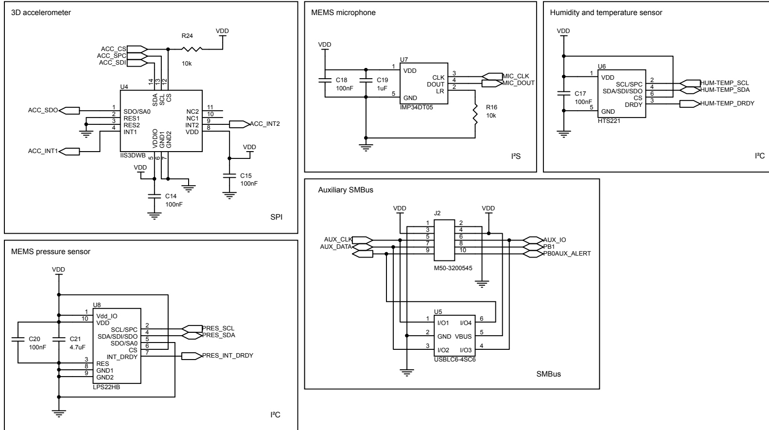
Figure 73. STEVAL-IDP005V2 (main board) circuit schematic - sensors
