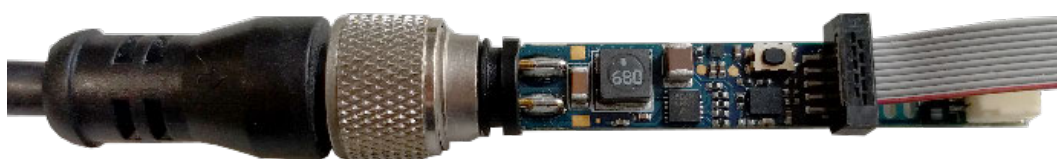
Figure 22. IO-Link and SWD connection
