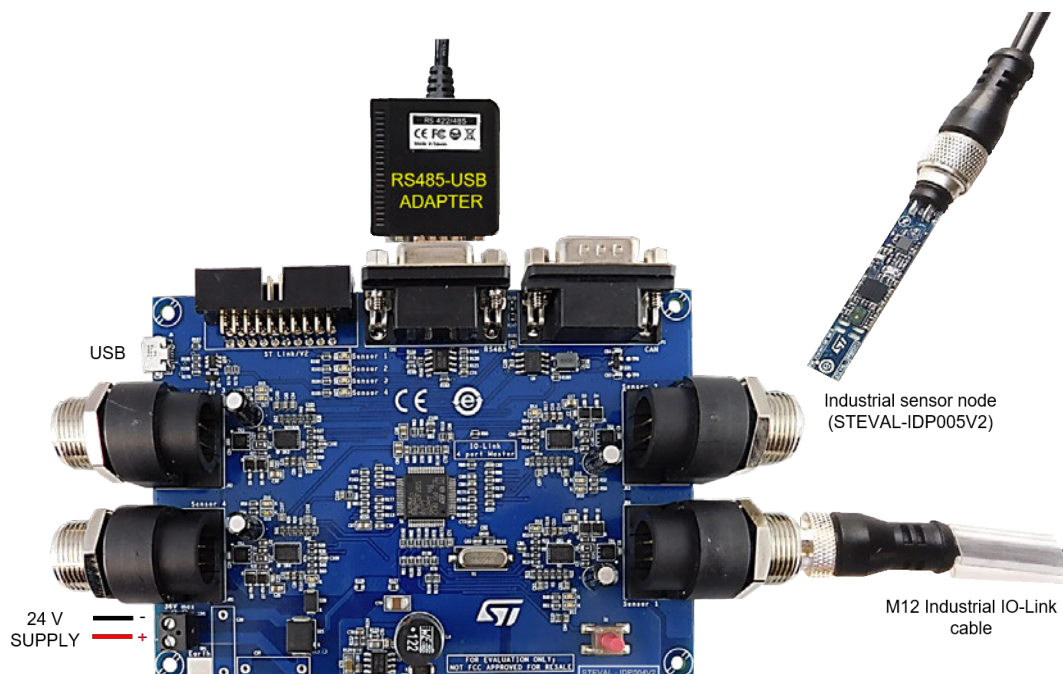
Figure 23. STEVAL-IDP004V2 and STEVAL-IDP005V2 connections
