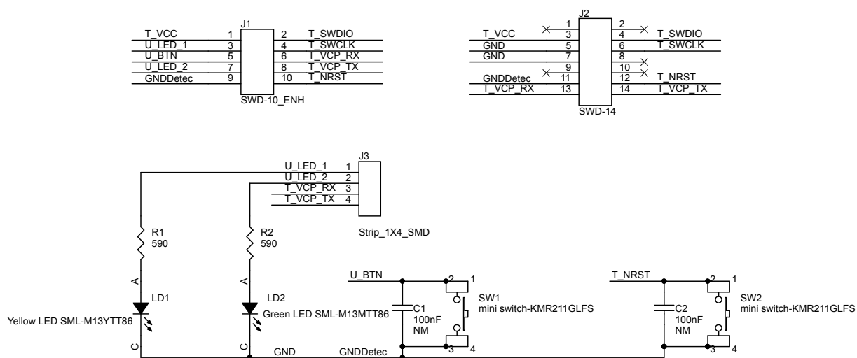
Figure 15. STEVAL-UKI001V2 schematic
