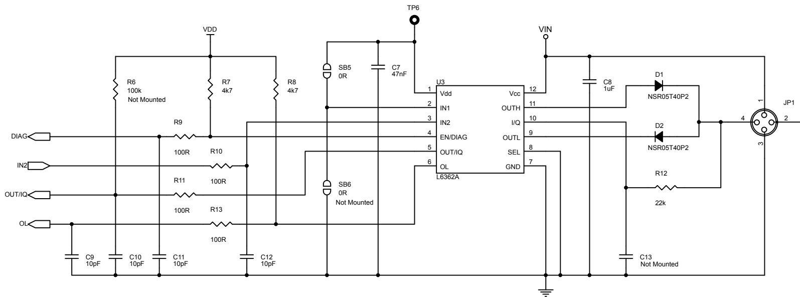
Figure 72. STEVAL-IDP005V2 (main board) circuit schematic - IO-Link
