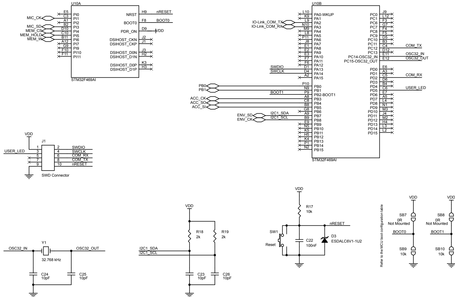
Figure 75. STEVAL-IDP005V2 (main board) circuit schematic - microcontroller (1 of 2)
