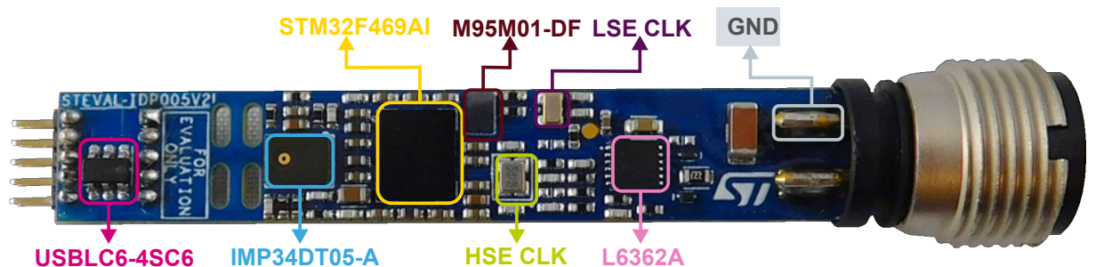
Figure 4. Industrial sensor node - bottom view
