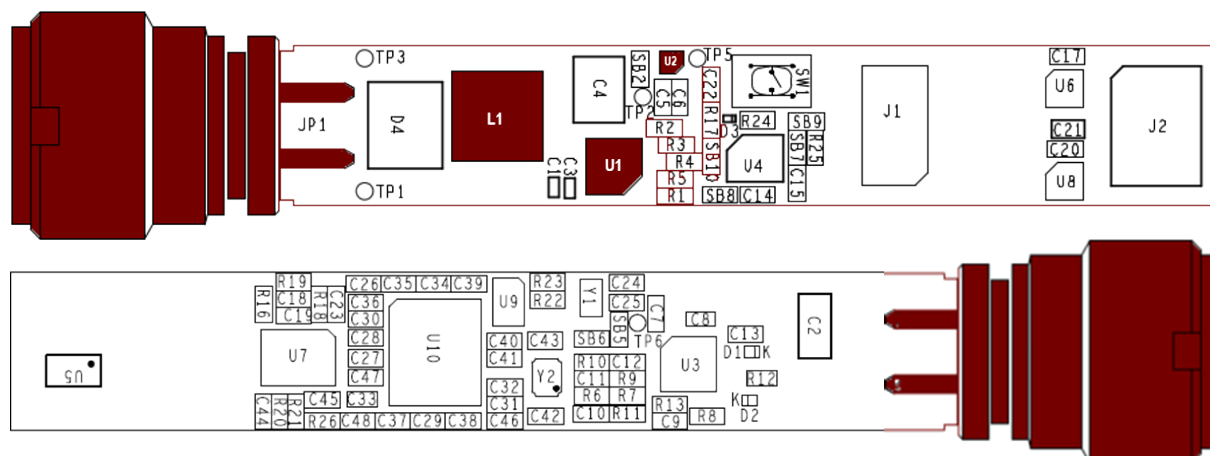
Figure 8. Power management system
