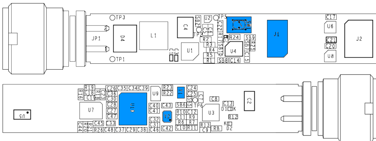
Figure 9. Microcontroller subsystem
