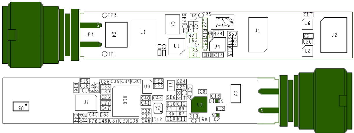
Figure 13. IO-Link subsystem
