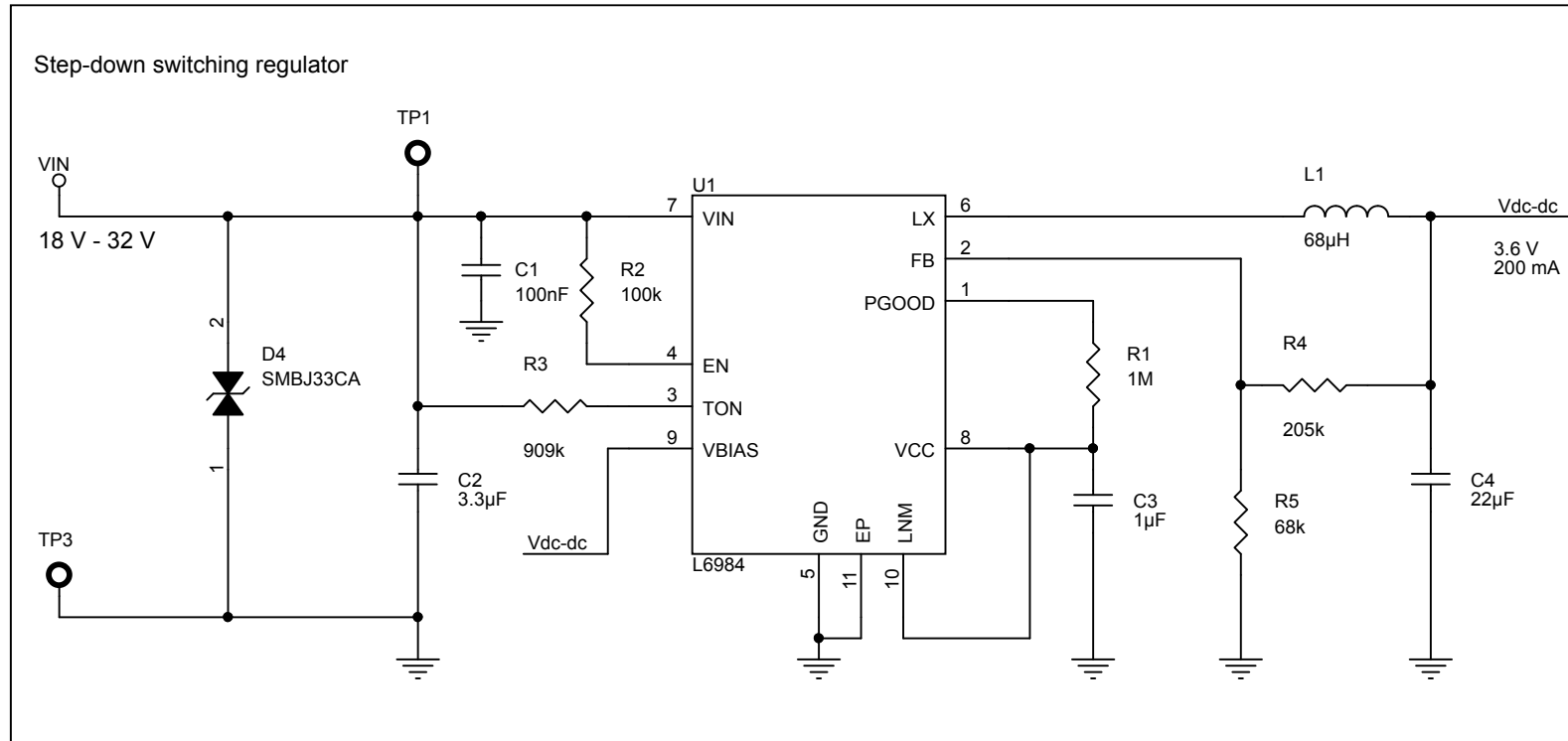
Figure 71. STEVAL-IDP005V2 (main board) circuit schematic - power management
