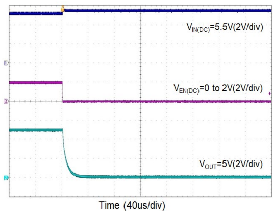
Enable Turn-Off Response ( V_{OUT}=5.0V )
