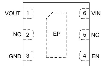
W-DFN2020-6 (SWP) (Type A1)
