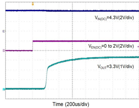
Enable Turn-On Response ( V_{OUT}=3.3V )
