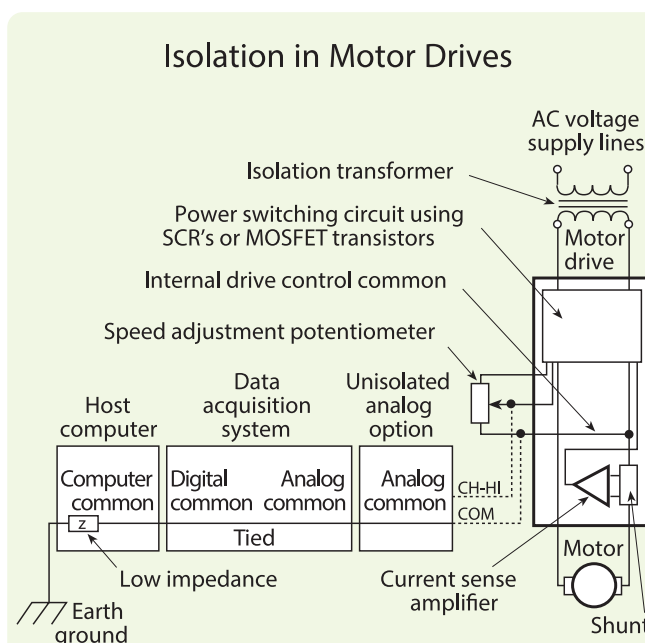
Fig. 10.12. Common-mode voltage is defined as the voltage between a signal and the localized common, which is usually earth ground. Common-mode voltages can be quite high, depending on the signal source. For example, a current sensing shunt in a dc motor drive might be expected to be at line-voltage potential, although the actual signal level is less than 50 mV across the shunt terminals. Measurement techniques for small signals at high common mode potentials call for isolation.
