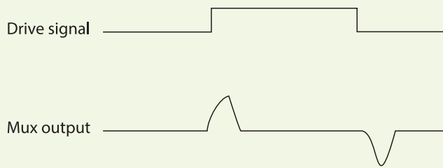
Fig. 5.03B. Analog-switching devices can produce spikes in the MUX output during level transitions in the drive signal. This is called charge-injection effect and can be minimized with low source impedance.
