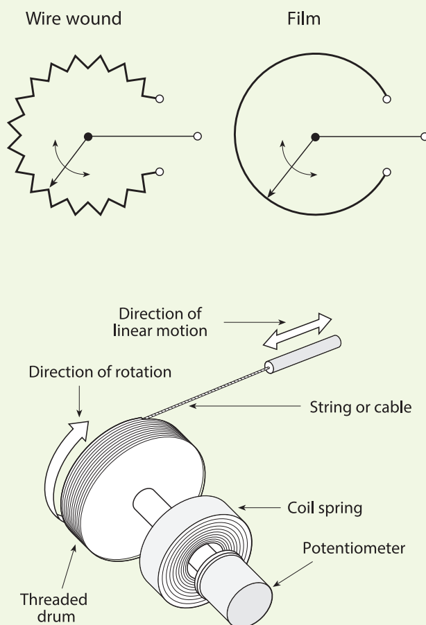
Fig. 9.01. String potentiometers occupy relatively little overall space in a machine installation or device under test. In some applications where a sensor cannot be mounted on the device being measured, the potentiometer may be conveniently located some distance from the test bed without sacrificing accuracy or repeatability.
