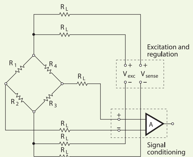
Fig. 4.18. The Kelvin connection eliminates lead resistance from altering the excitation voltage by using a second pair of wires. The measuring device has relatively high input impedance so it does not draw current and develop a voltage drop across its leads that would add an error.
