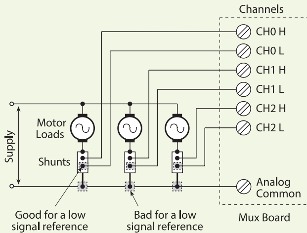
Fig. 4.05. High dc currents are often measured with shunts using differential inputs sharing a common ground.
