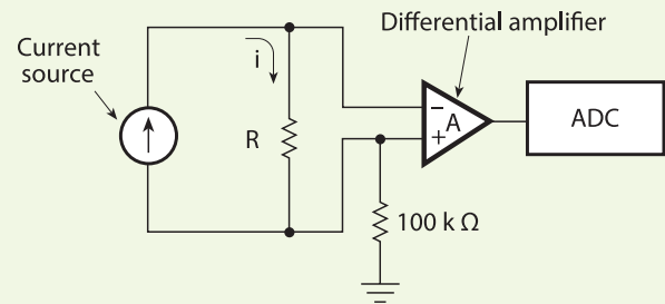
Fig. 4.06. Sensors with 4 to 20 mA outputs are typically placed in series with a resistor to develop a voltage. The resistor is then connected to the input of a differential amplifier to measure the voltage drop.
