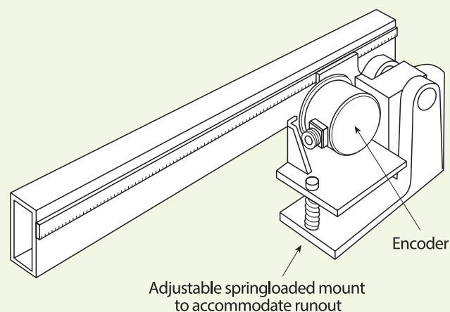
Fig. 9.05. A rack and pinion sensor assembly should have a flexible mount to compensate the combined runout error. In a machine application, the sensor should be protected from metal chips and other foreign objects to ensure measurement accuracy.
