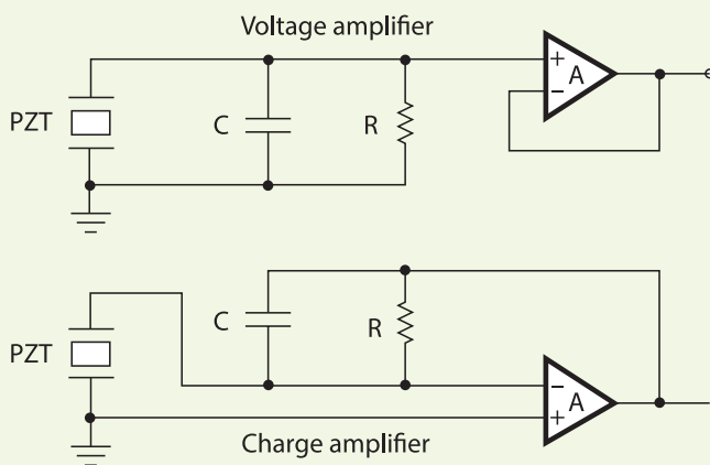
Fig. 8.03. A high-gain op amp isolates the sensor's output voltage from the effect of signal cable capacitance and lets the amplifier reside several meters away from the sensor.
