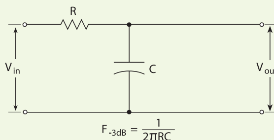
Fig. 10.14. Passive single pole filters are moderately effective in passing a band of frequencies that contain the measured signal, while attenuating other frequencies containing noise.
