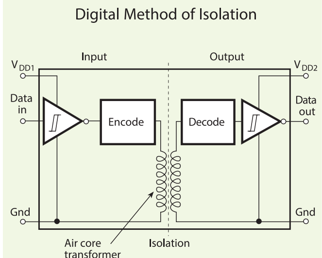
Fig. 5.25. Yet another isolation method specifically intended for digital circuits employs a high-speed CMOS encoder and decoder at the input and output, coupled with a monolithic air-core transformer.
