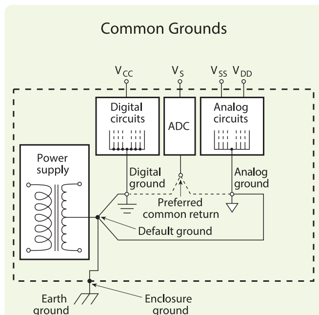
Fig. 10.02. Significant current fed to multiple circuits should have individual return paths to a common ground or negative terminal. This reduces the risk of voltage drops developing over long ground runs or lead wires that could become input (error) signals to other circuits.
