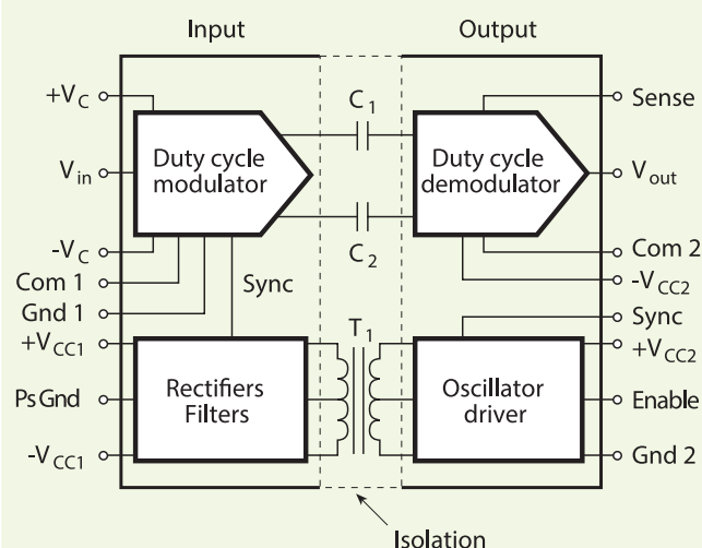
Fig. 10.10. Low-cost isolation amplifiers couple dc signals by modulating the signal, coupling its ac equivalent through a substrate capacitor connecting the stages, and then demodulating the signal to restore it to its original dc value.
