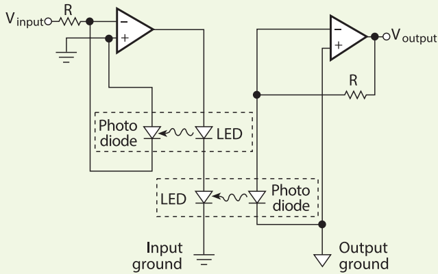
Fig. 4.17. When making high common-mode voltage measurements, optical couplers provide a convenient and safe means for connecting the voltage to data acquisition systems.
