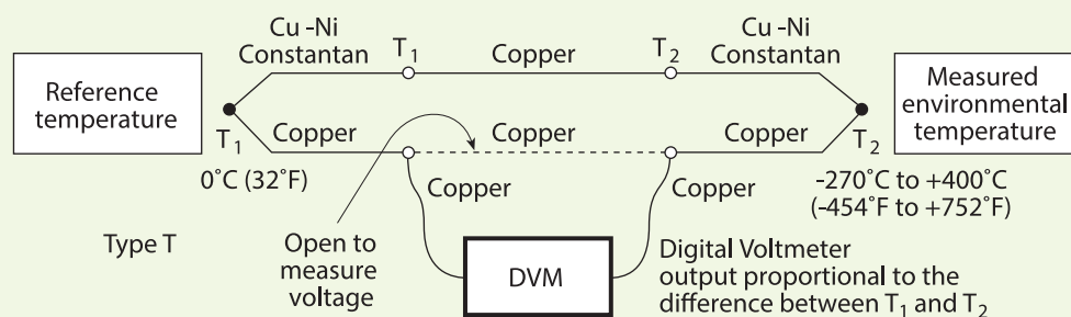
Fig. 6.01. A basic thermocouple measurement system requires two sensors, one for the environment under measurement and the other, a reference junction, normally held to 0°C (32°F). Type-T is one of the dozen or more common thermocouples frequently used in general-purpose temperature measuring applications. It is made of copper and constantan metals and typically operates from -270 to +400°C or -454 to +752°F.
