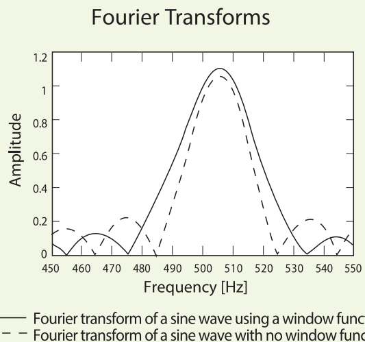
Fig. 3.11. A Fourier Transform is shown with and without a window function.
