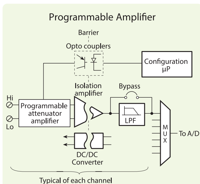
Fig. 10.11 All three techniques of isolation are used in a multi-channel, programmable amplifier. Optical devices couple digital signals, capacitors couple analog signals, and the dc/dc converter supplies power to the isolated side.
