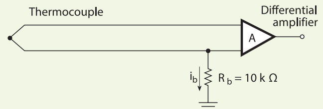
Fig. 4.14. The resistor is necessary for at least one input to provide the path to ground for amplifier bias currents.
