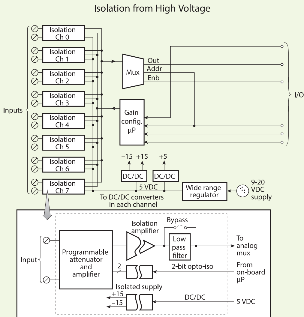
Fig. 5.34. The isolated voltage-input modules let data acquisition systems isolate several channels of analog input, up to 500 V channel-to-channel and channel-to-system.
