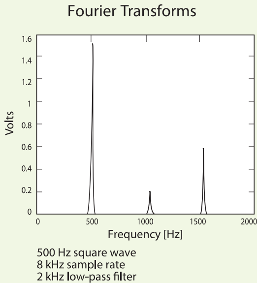
Fig. 3.10. The Fourier Transform of a 500 Hz square wave is sampled at 8 kHz with a low-pass filter cutoff at 2 kHz.
