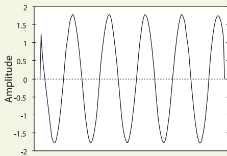
Fig. 3.12. The frequency information obtained from a measurement can be incorrect when the waveform contains abrupt beginning or ending points.
