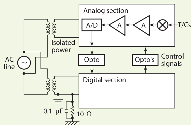
Fig. 10.09. Optical devices are the most widely used component for coupling signals across high-potential barriers and for low-level signals that are prone to the electrical noise typically coupled through different ground potentials.
