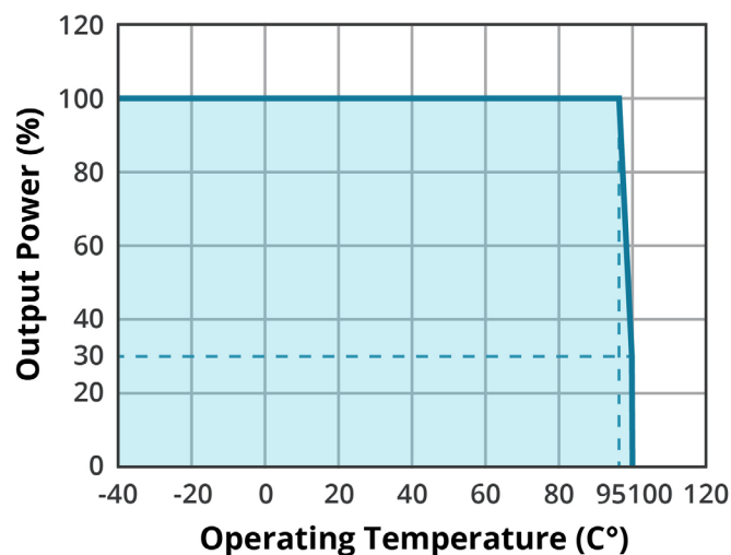
TEMPERATURE DERATING CURVE (natural convection 20 LFM) DHP1-3-S12-M & DHP1-3-S15-M
