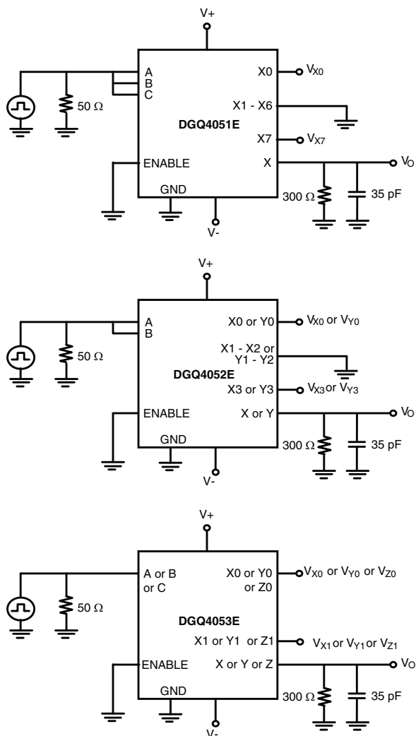
Fig. 1 - Transition Time
