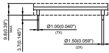
SIDE VIEW ( without heat spreader )
